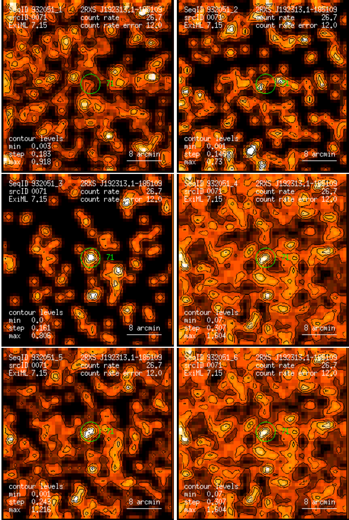
Figure 71: RASS 932051: detection 0071: band rate images, Gaussian filter: (1) PSPC channels 11 – 41, (2) 52 – 90, (3) 91 – 201, (4) 11 – 235, (5) 52 – 201, (6) 11 – 201. Broad band rates in counts/ks. Band rate contour levels in counts/ks/arcmin 2 .
