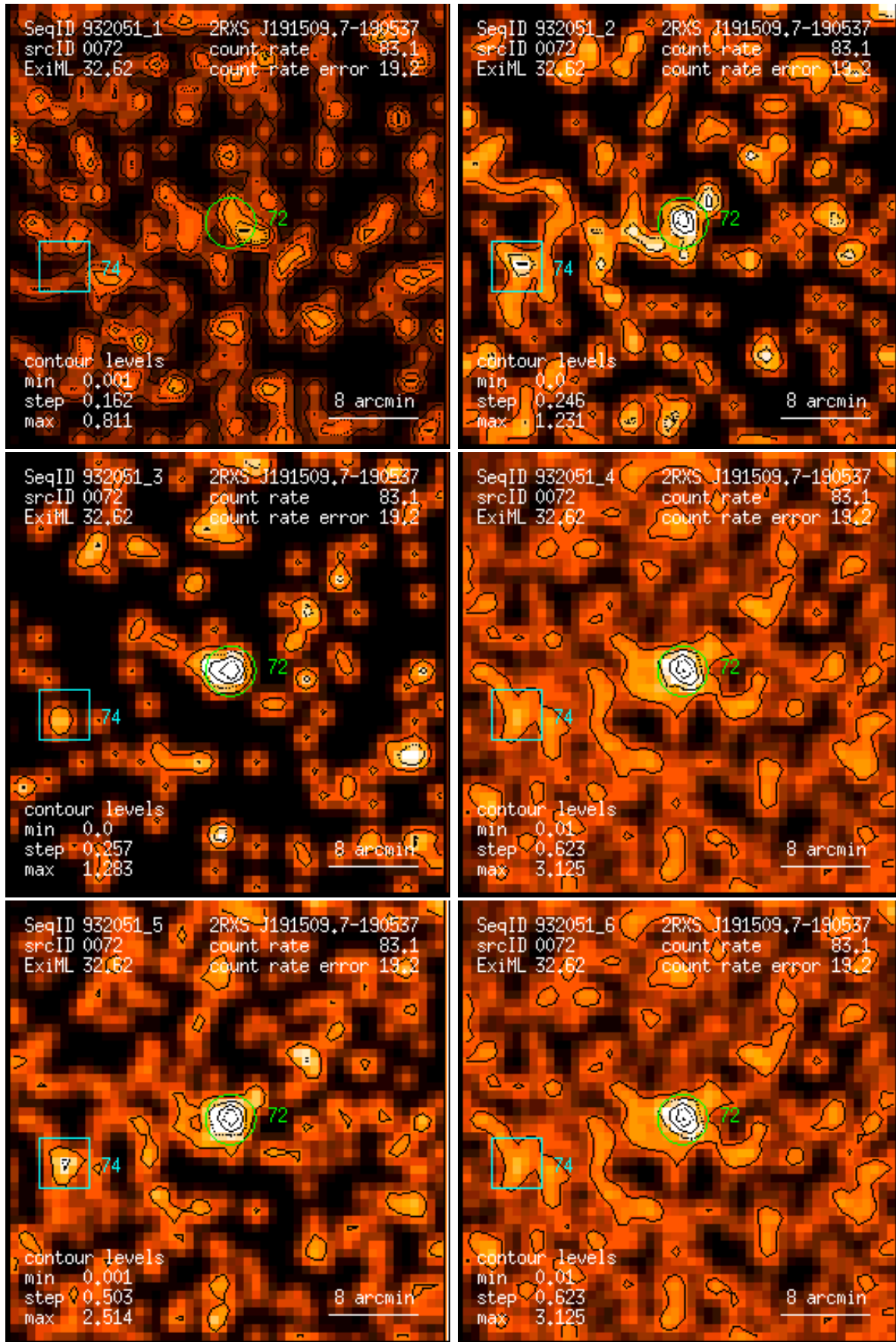
Figure 72: RASS 932051: detection 0072: band rate images, Gaussian filter: (1) PSPC channels 11 – 41, (2) 52 – 90, (3) 91 – 201, (4) 11 – 235, (5) 52 – 201, (6) 11 – 201. Broad band rates in counts/ks. Band rate contour levels in counts/ks/arcmin 2 .
