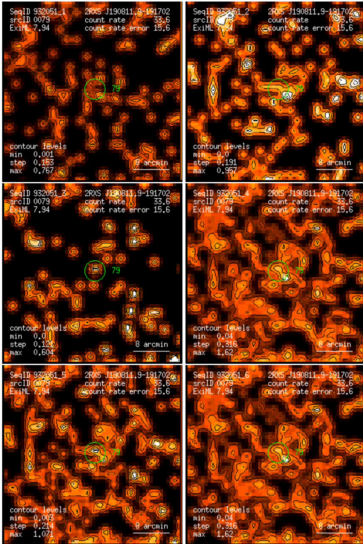
Figure 79: RASS 932051: detection 0079: band rate images, Gaussian filter: (1) PSPC channels 11 – 41, (2) 52 – 90, (3) 91 – 201, (4) 11 – 235, (5) 52 – 201, (6) 11 – 201. Broad band rates in counts/ks. Band rate contour levels in counts/ks/arcmin 2 .
