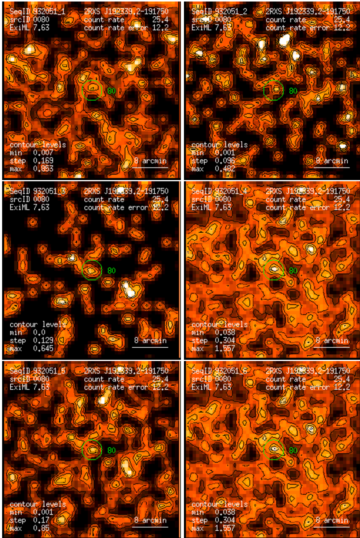
Figure 80: RASS 932051: detection 0080: band rate images, Gaussian filter: (1) PSPC channels 11 – 41, (2) 52 – 90, (3) 91 – 201, (4) 11 – 235, (5) 52 – 201, (6) 11 – 201. Broad band rates in counts/ks. Band rate contour levels in counts/ks/arcmin 2 .
