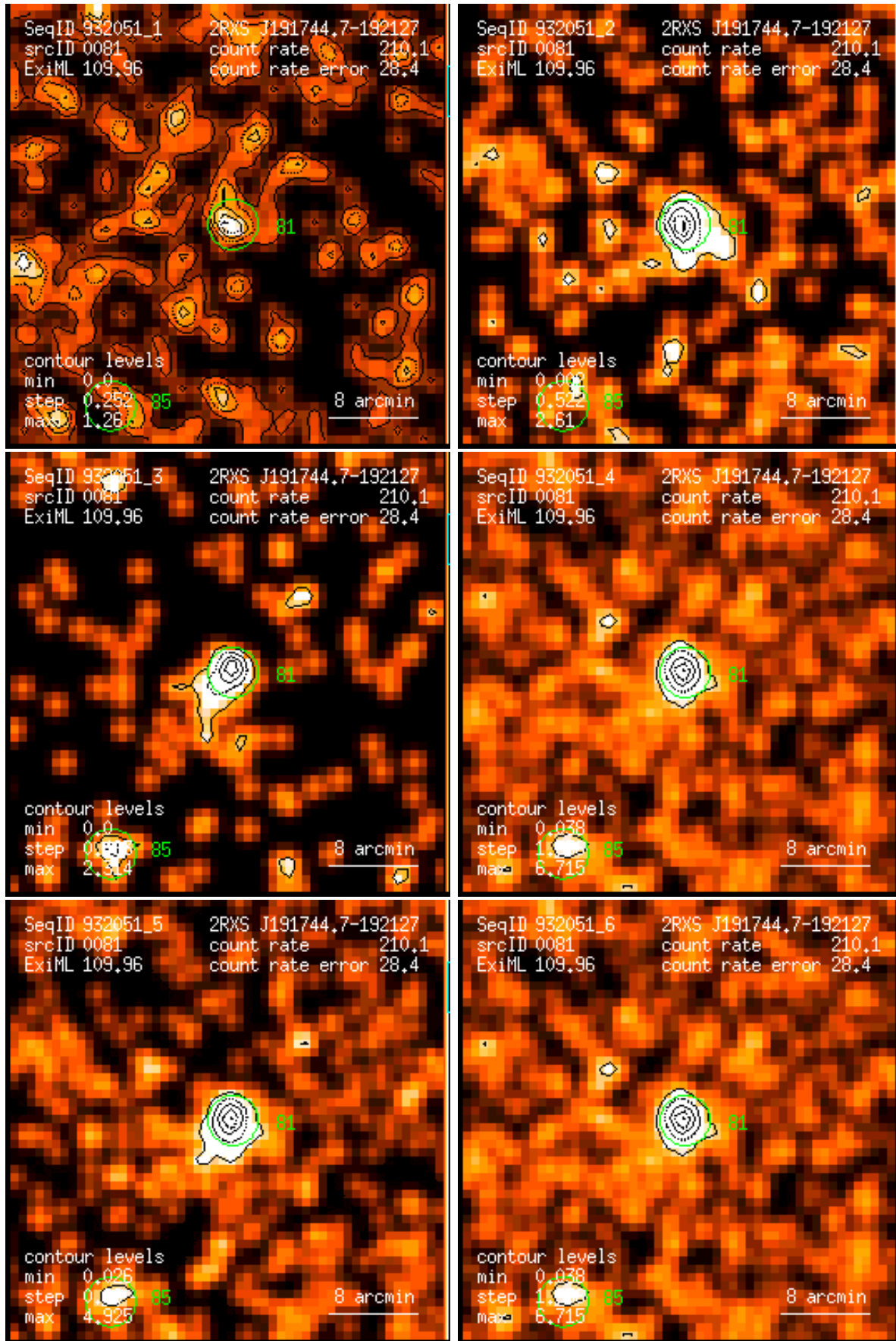
Figure 81: RASS 932051: detection 0081: band rate images, Gaussian filter: (1) PSPC channels 11 – 41, (2) 52 – 90, (3) 91 – 201, (4) 11 – 235, (5) 52 – 201, (6) 11 – 201. Broad band rates in counts/ks. Band rate contour levels in counts/ks/arcmin 2 .
