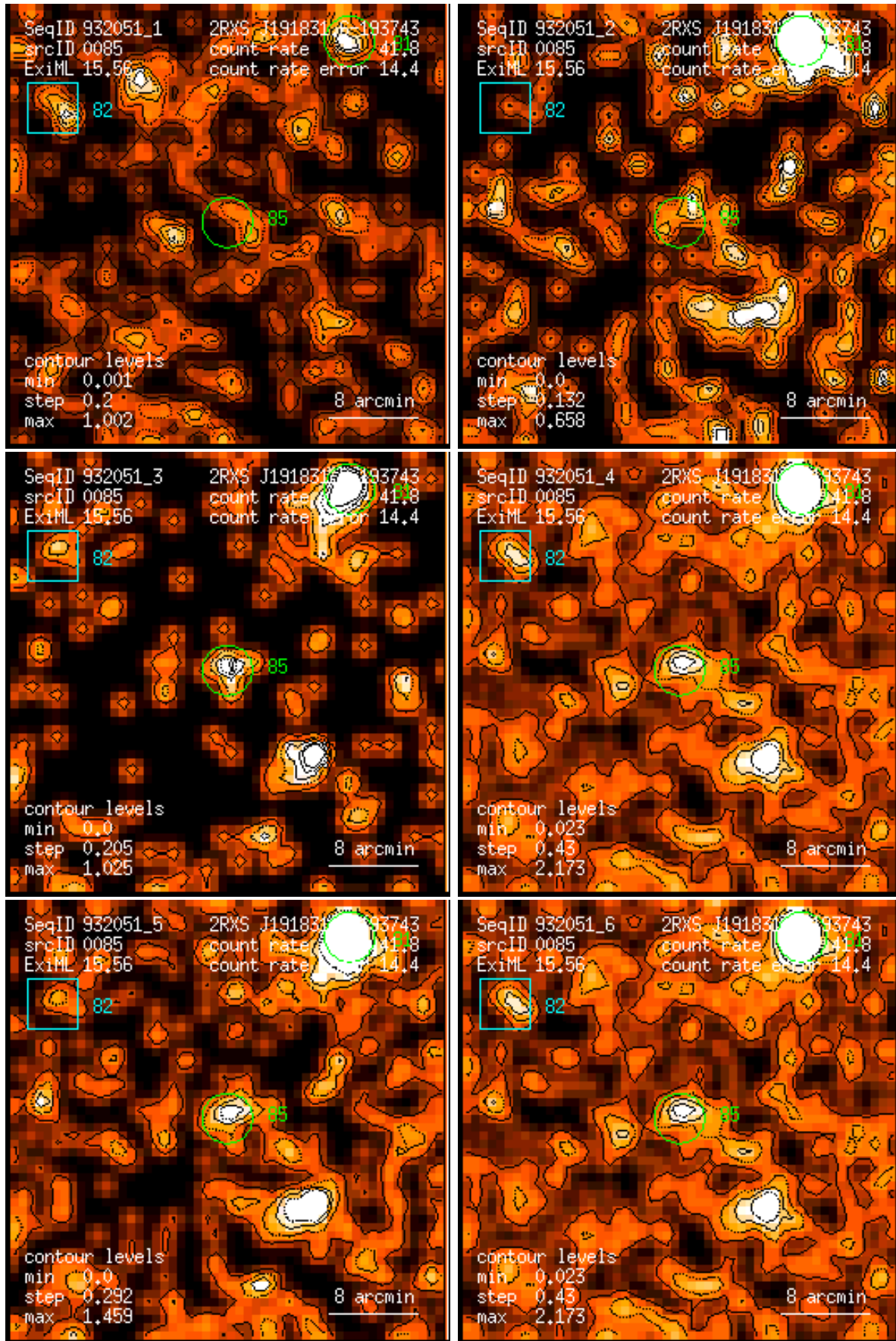
Figure 85: RASS 932051: detection 0085: band rate images, Gaussian filter: (1) PSPC channels 11 – 41, (2) 52 – 90, (3) 91 – 201, (4) 11 – 235, (5) 52 – 201, (6) 11 – 201. Broad band rates in counts/ks. Band rate contour levels in counts/ks/arcmin 2 .
