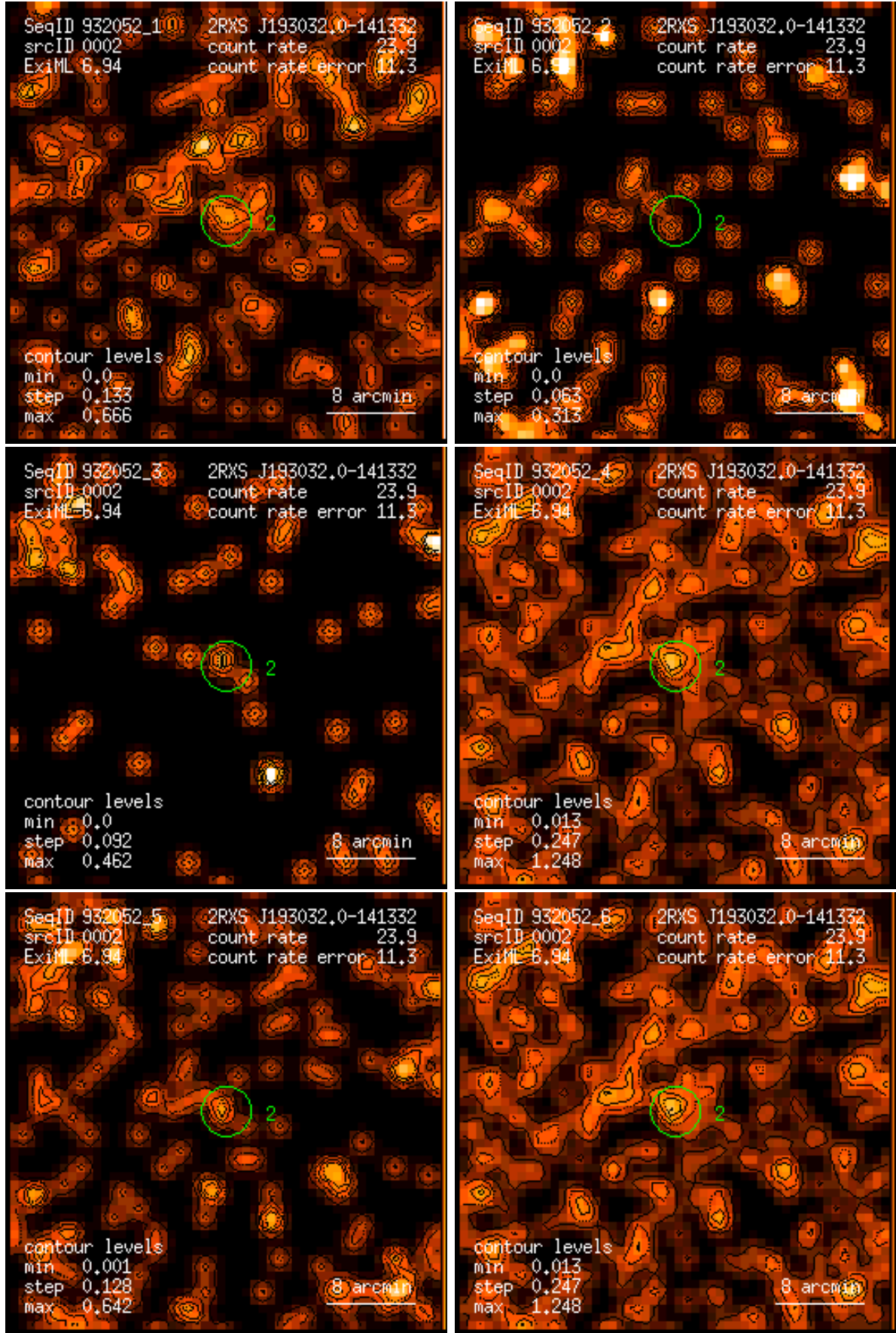
Figure 2: RASS 932052: detection 0002: band rate images, Gaussian filter: (1) PSPC channels 11 – 41, (2) 52 – 90, (3) 91 – 201, (4) 11 – 235, (5) 52 – 201, (6) 11 – 201. Broad band rates in counts/ks. Band rate contour levels in counts/ks/arcmin 2 .
