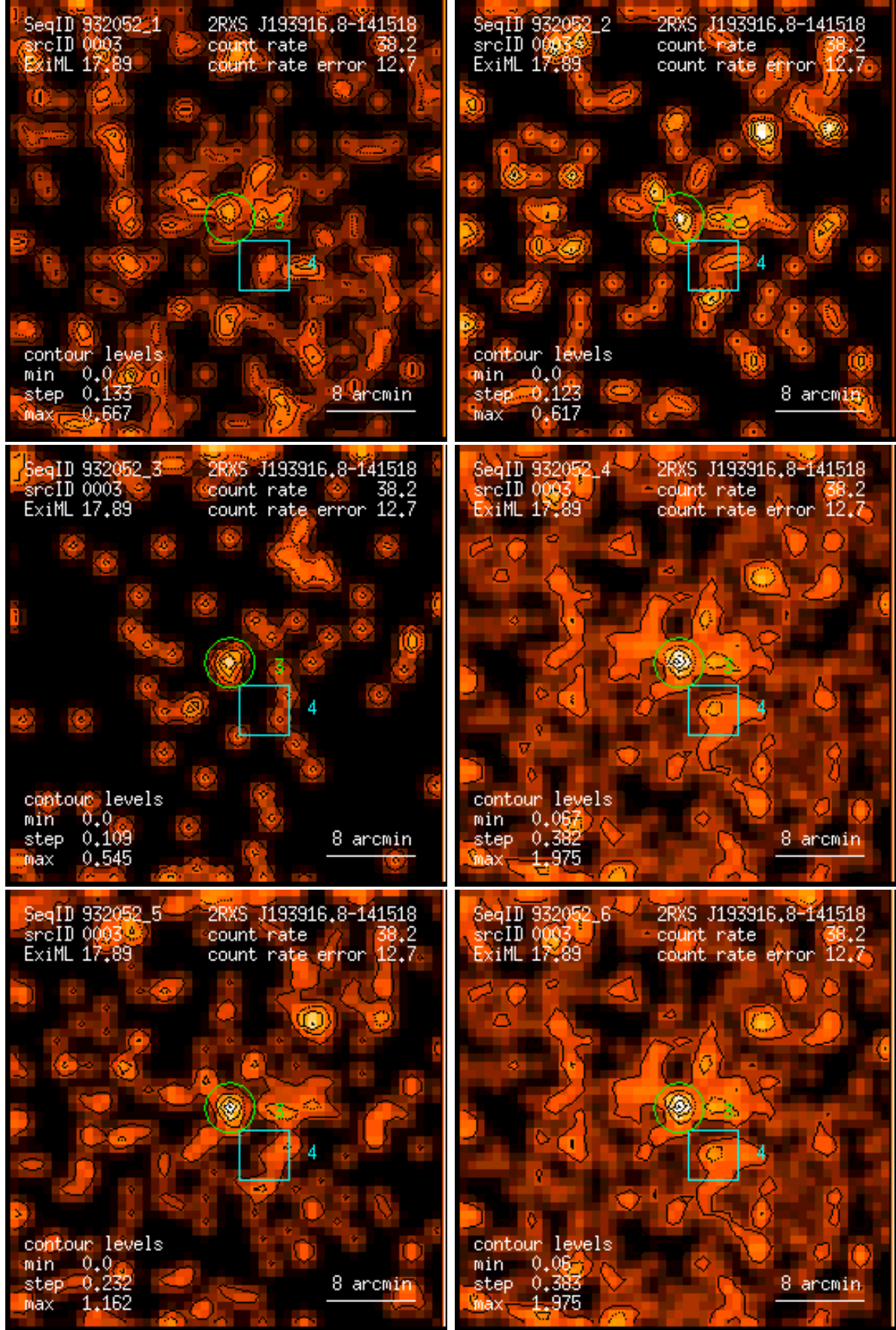
Figure 3: RASS 932052: detection 0003: band rate images, Gaussian filter: (1) PSPC channels 11 – 41, (2) 52 – 90, (3) 91 – 201, (4) 11 – 235, (5) 52 – 201, (6) 11 – 201. Broad band rates in counts/ks. Band rate contour levels in counts/ks/arcmin 2 .
