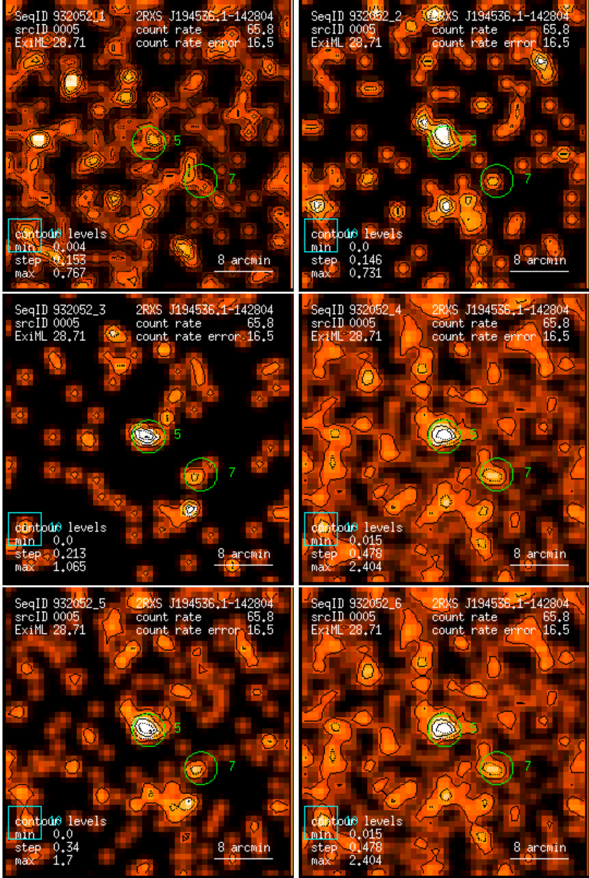
Figure 5: RASS 932052: detection 0005: band rate images, Gaussian filter: (1) PSPC channels 11 – 41, (2) 52 – 90, (3) 91 – 201, (4) 11 – 235, (5) 52 – 201, (6) 11 – 201. Broad band rates in counts/ks. Band rate contour levels in counts/ks/arcmin 2 .
