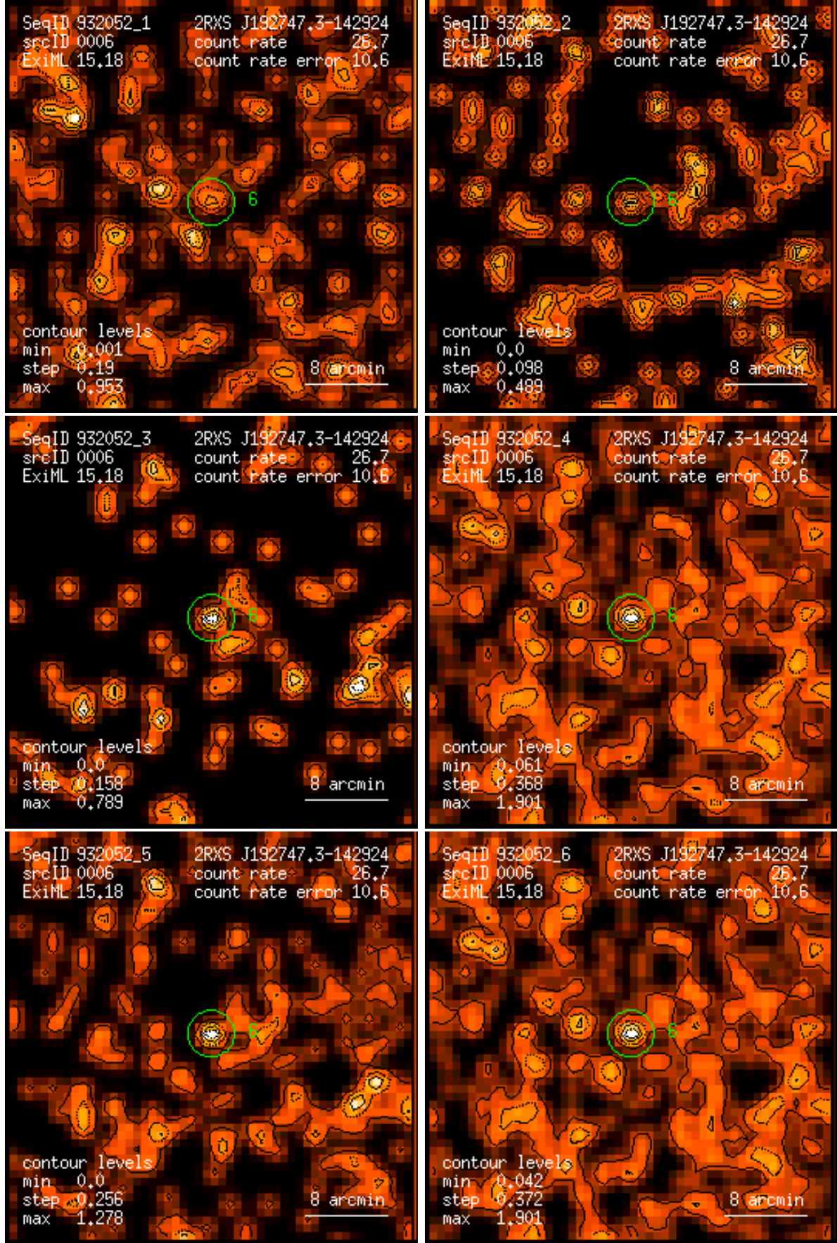
Figure 6: RASS 932052: detection 0006: band rate images, Gaussian filter: (1) PSPC channels 11 – 41, (2) 52 – 90, (3) 91 – 201, (4) 11 – 235, (5) 52 – 201, (6) 11 – 201. Broad band rates in counts/ks. Band rate contour levels in counts/ks/arcmin 2 .
