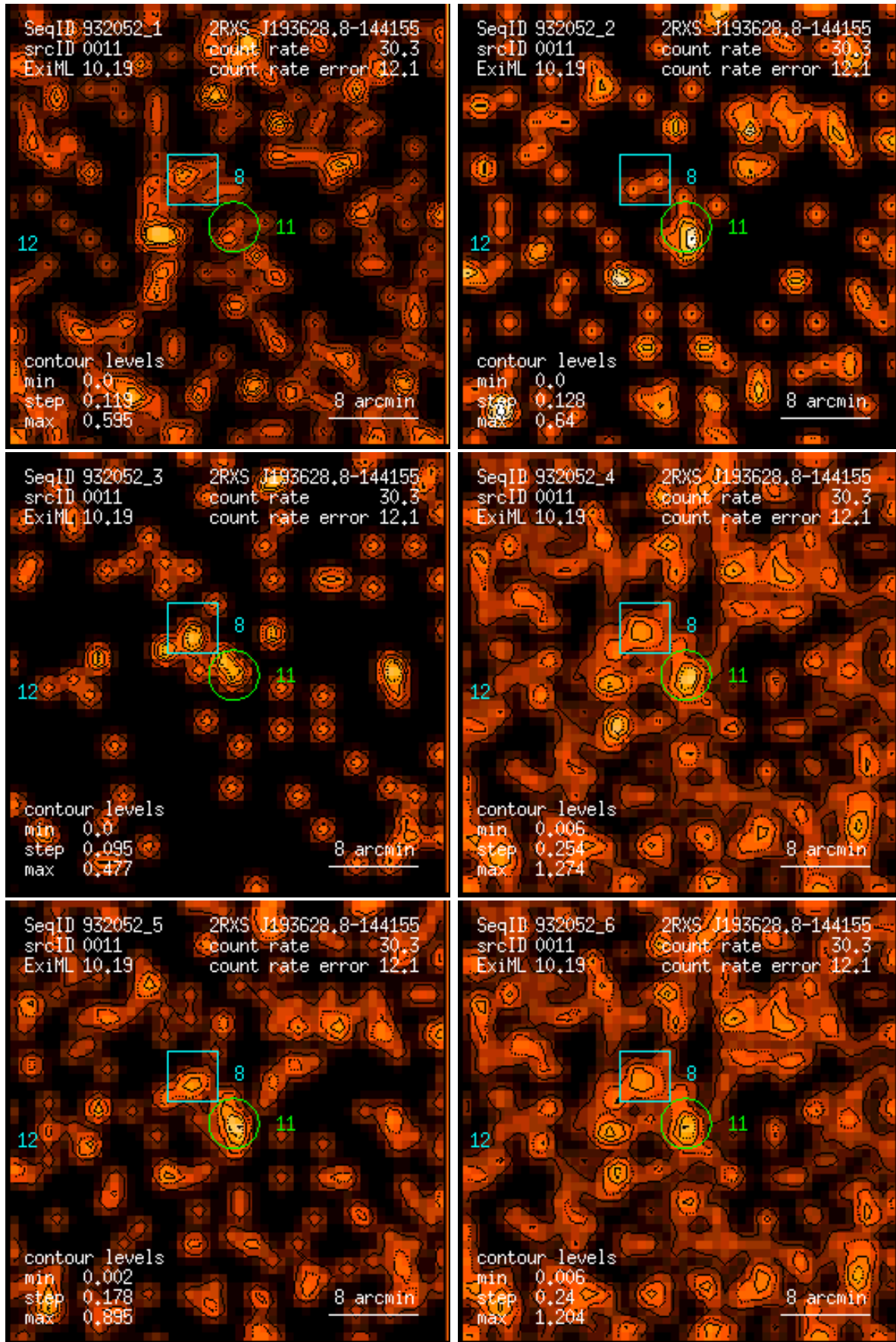
Figure 11: RASS 932052: detection 0011: band rate images, Gaussian filter: (1) PSPC channels 11 – 41, (2) 52 – 90, (3) 91 – 201, (4) 11 – 235, (5) 52 – 201, (6) 11 – 201. Broad band rates in counts/ks. Band rate contour levels in counts/ks/arcmin 2 .
