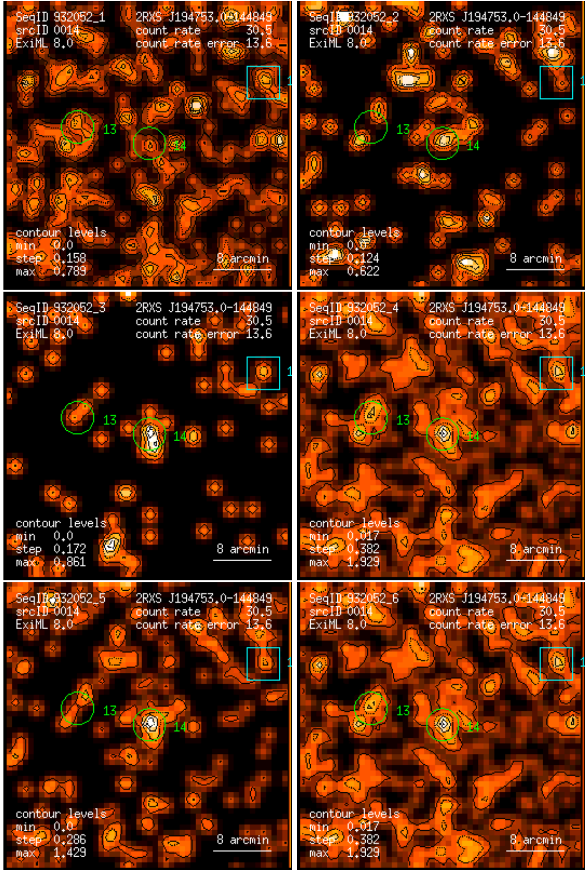
Figure 14: RASS 932052: detection 0014: band rate images, Gaussian filter: (1) PSPC channels 11 – 41, (2) 52 – 90, (3) 91 – 201, (4) 11 – 235, (5) 52 – 201, (6) 11 – 201. Broad band rates in counts/ks. Band rate contour levels in counts/ks/arcmin 2 .
