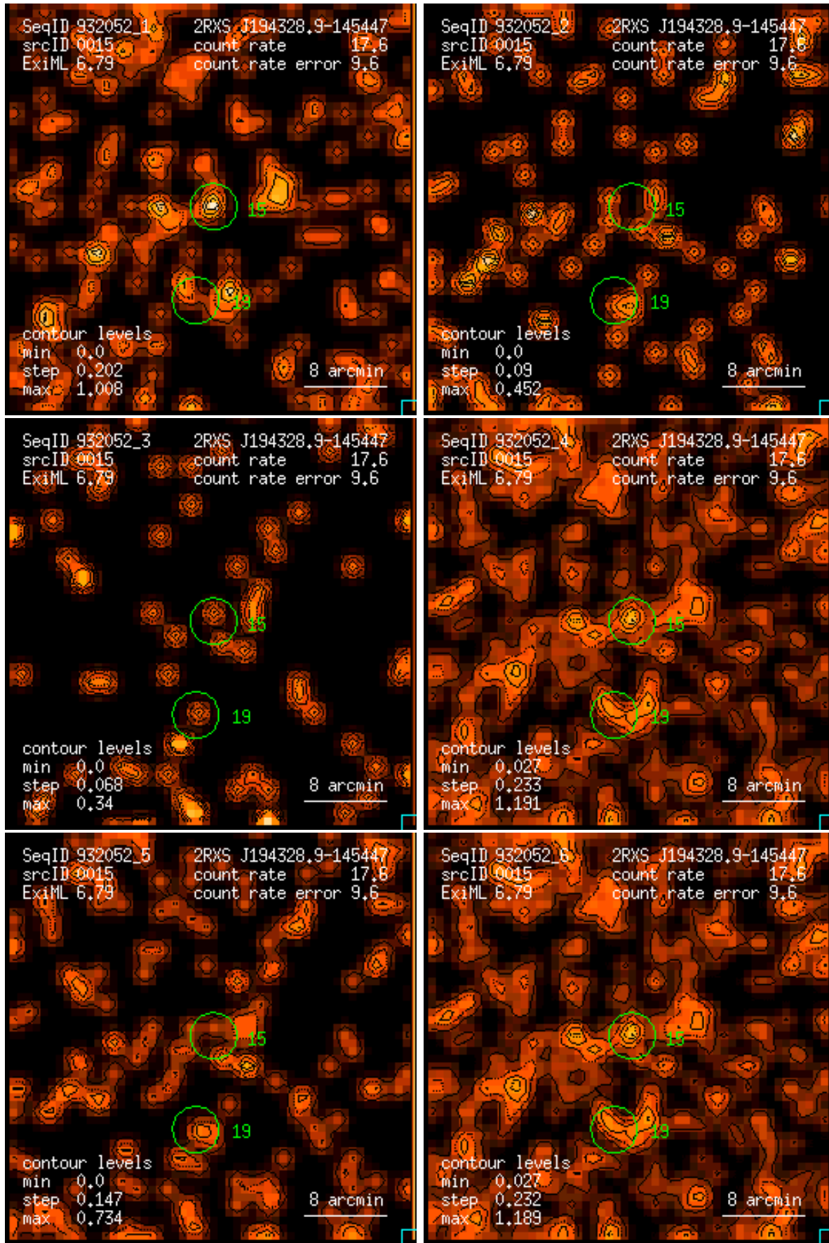
Figure 15: RASS 932052: detection 0015: band rate images, Gaussian filter: (1) PSPC channels 11 – 41, (2) 52 – 90, (3) 91 – 201, (4) 11 – 235, (5) 52 – 201, (6) 11 – 201. Broad band rates in counts/ks. Band rate contour levels in counts/ks/arcmin 2 .
