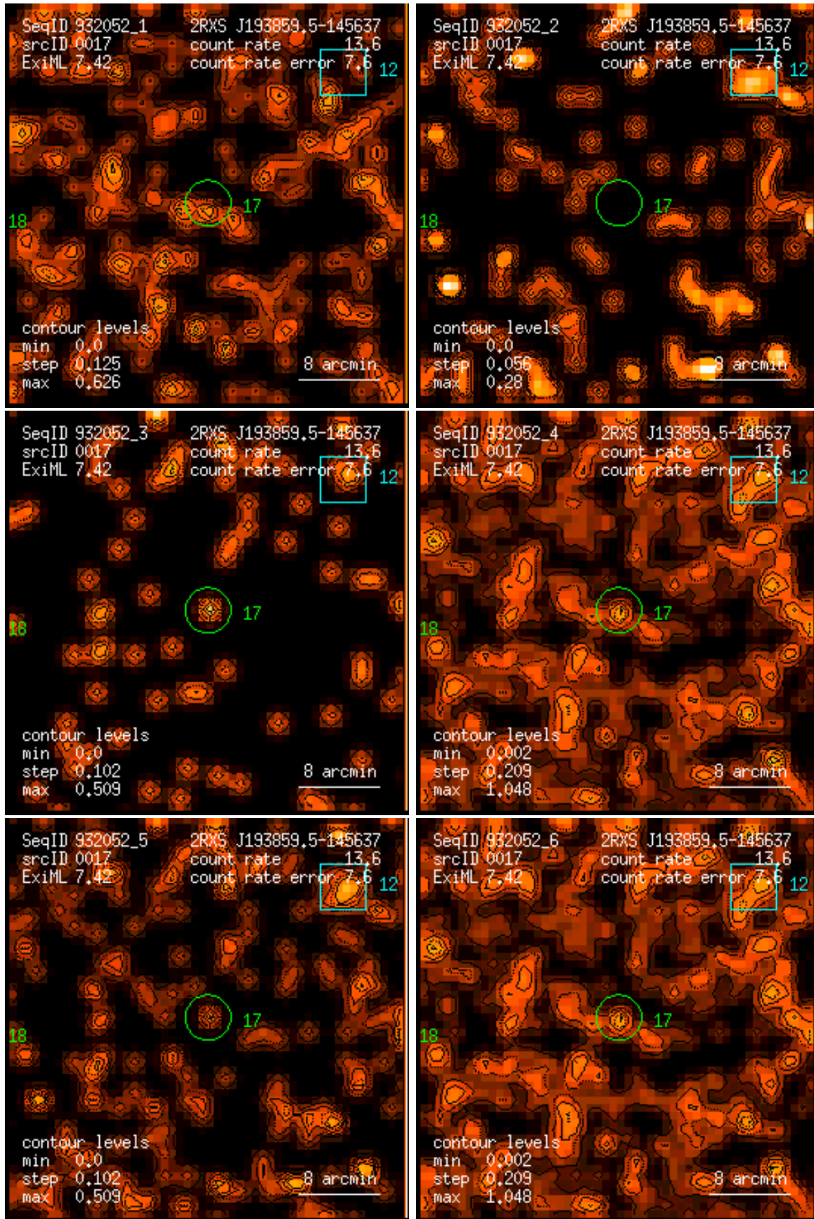
Figure 17: RASS 932052: detection 0017: band rate images, Gaussian filter: (1) PSPC channels 11 – 41, (2) 52 – 90, (3) 91 – 201, (4) 11 – 235, (5) 52 – 201, (6) 11 – 201. Broad band rates in counts/ks. Band rate contour levels in counts/ks/arcmin 2 .
