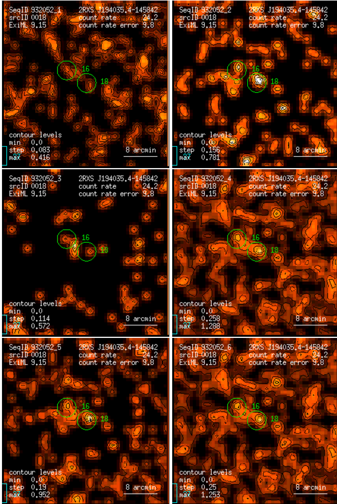
Figure 18: RASS 932052: detection 0018: band rate images, Gaussian filter: (1) PSPC channels 11 – 41, (2) 52 – 90, (3) 91 – 201, (4) 11 – 235, (5) 52 – 201, (6) 11 – 201. Broad band rates in counts/ks. Band rate contour levels in counts/ks/arcmin 2 .
