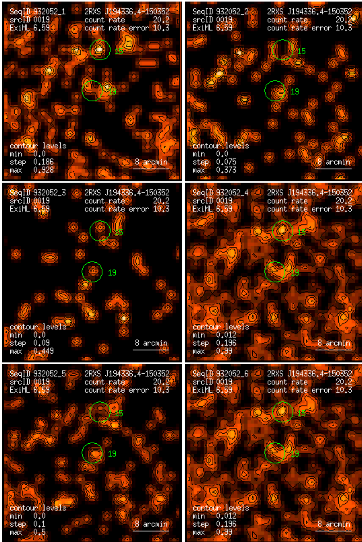
Figure 19: RASS 932052: detection 0019: band rate images, Gaussian filter: (1) PSPC channels 11 – 41, (2) 52 – 90, (3) 91 – 201, (4) 11 – 235, (5) 52 – 201, (6) 11 – 201. Broad band rates in counts/ks. Band rate contour levels in counts/ks/arcmin 2 .
