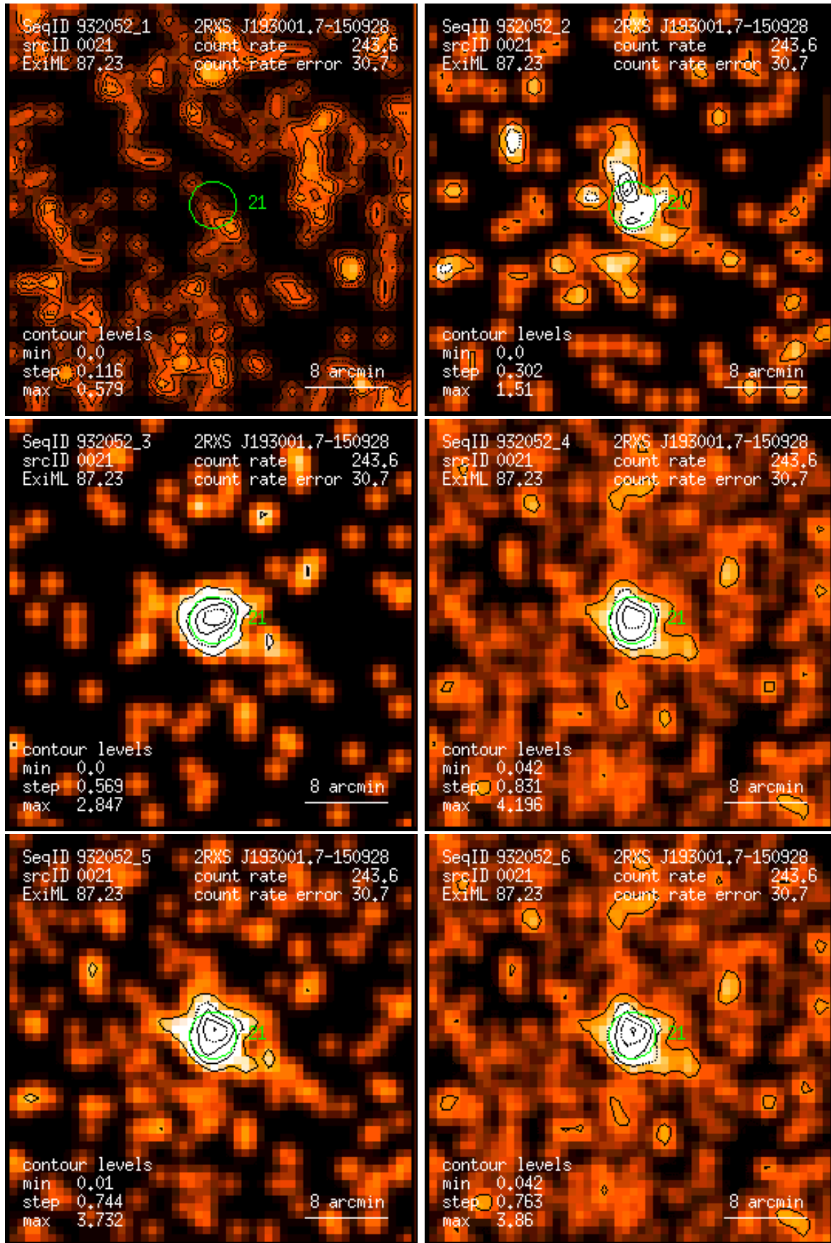
Figure 21: RASS 932052: detection 0021: band rate images, Gaussian filter: (1) PSPC channels 11 – 41, (2) 52 – 90, (3) 91 – 201, (4) 11 – 235, (5) 52 – 201, (6) 11 – 201. Broad band rates in counts/ks. Band rate contour levels in counts/ks/arcmin 2 .
