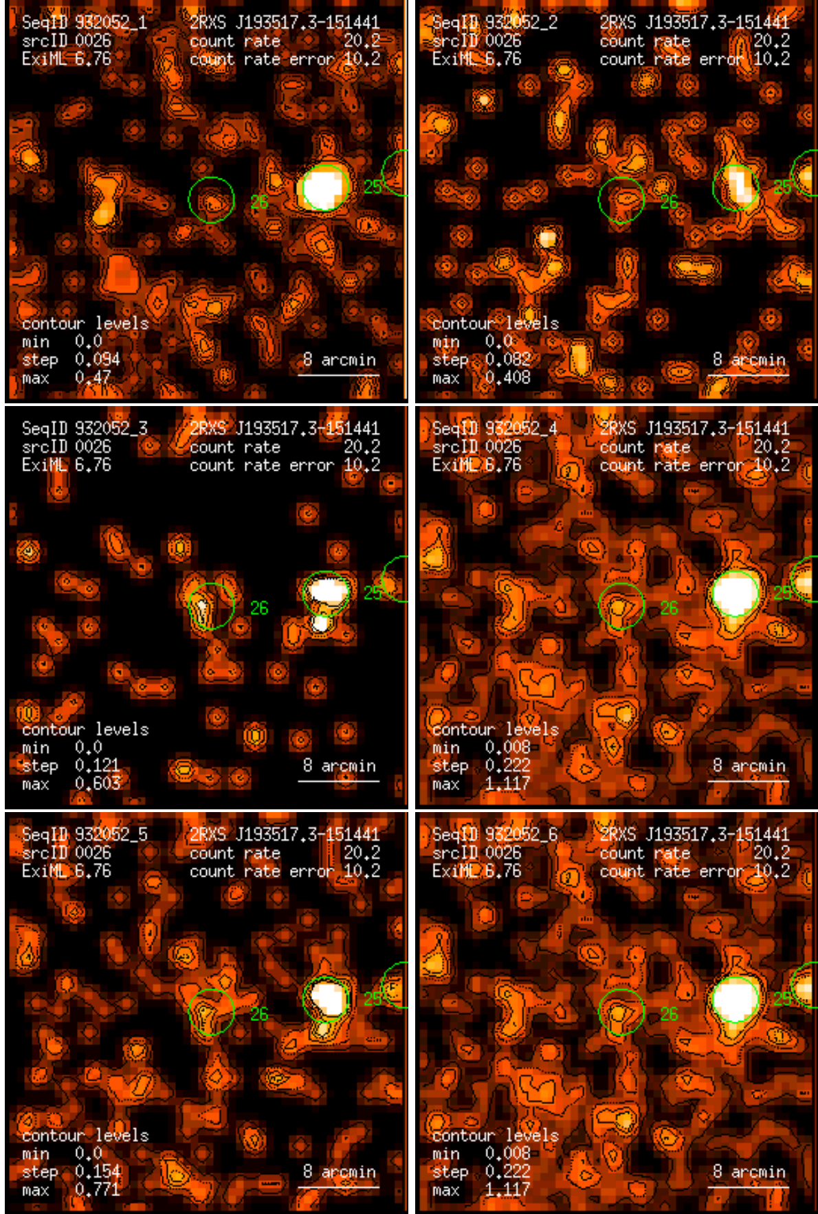
Figure 26: RASS 932052: detection 0026: band rate images, Gaussian filter: (1) PSPC channels 11 – 41, (2) 52 – 90, (3) 91 – 201, (4) 11 – 235, (5) 52 – 201, (6) 11 – 201. Broad band rates in counts/ks. Band rate contour levels in counts/ks/arcmin 2 .
