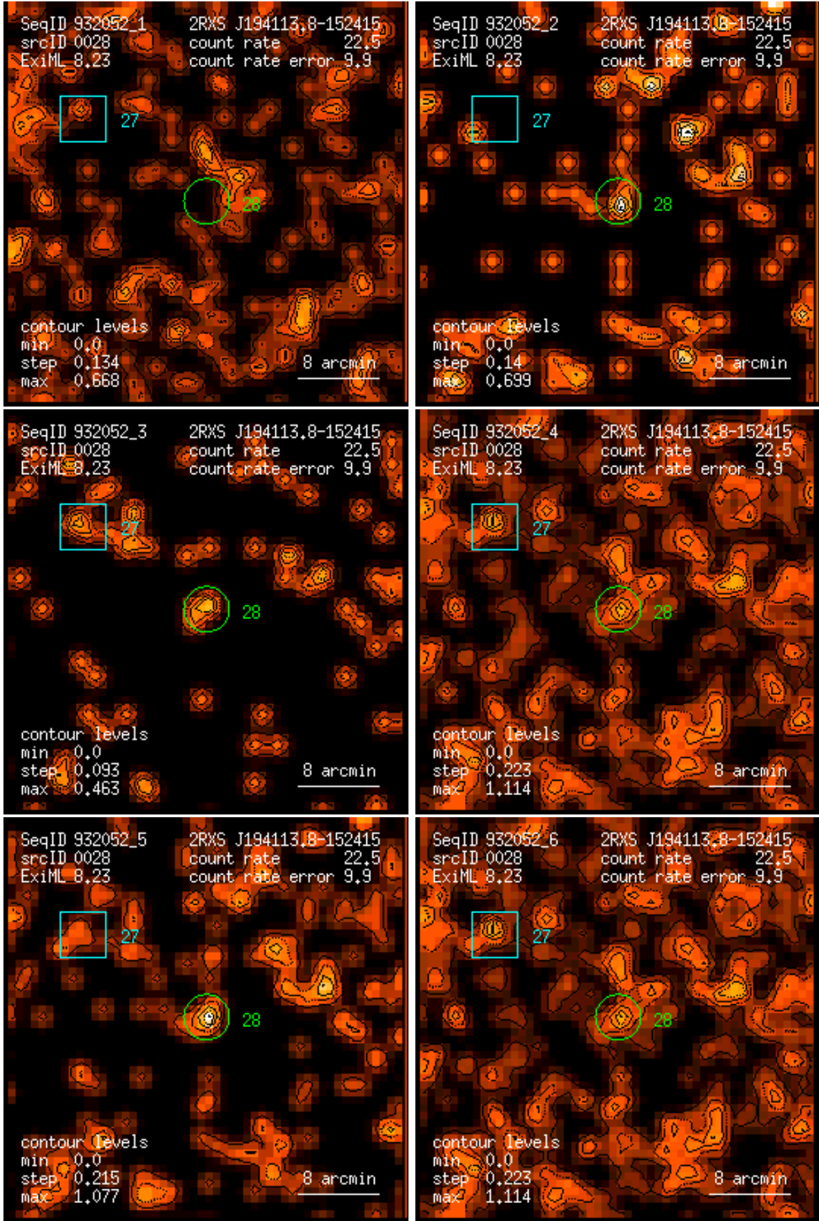
Figure 28: RASS 932052: detection 0028: band rate images, Gaussian filter: (1) PSPC channels 11 – 41, (2) 52 – 90, (3) 91 – 201, (4) 11 – 235, (5) 52 – 201, (6) 11 – 201. Broad band rates in counts/ks. Band rate contour levels in counts/ks/arcmin 2 .
