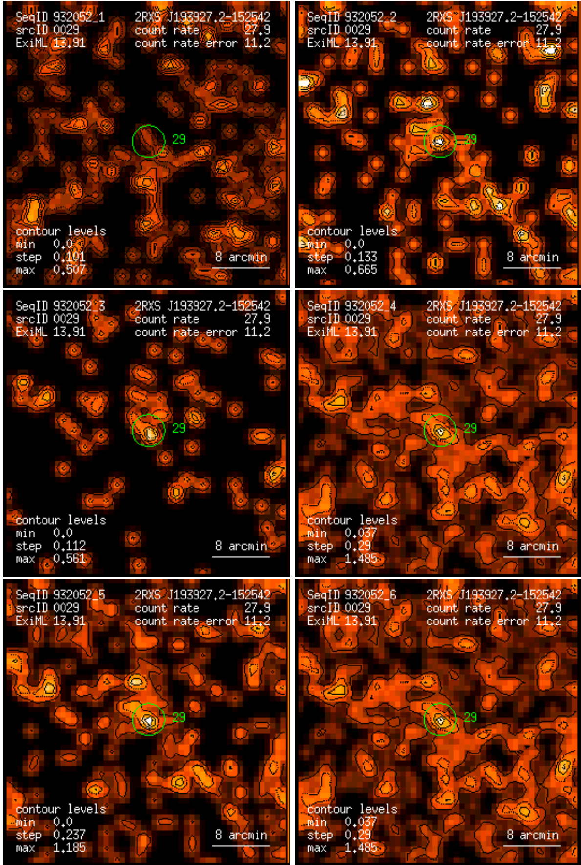
Figure 29: RASS 932052: detection 0029: band rate images, Gaussian filter: (1) PSPC channels 11 – 41, (2) 52 – 90, (3) 91 – 201, (4) 11 – 235, (5) 52 – 201, (6) 11 – 201. Broad band rates in counts/ks. Band rate contour levels in counts/ks/arcmin 2 .
