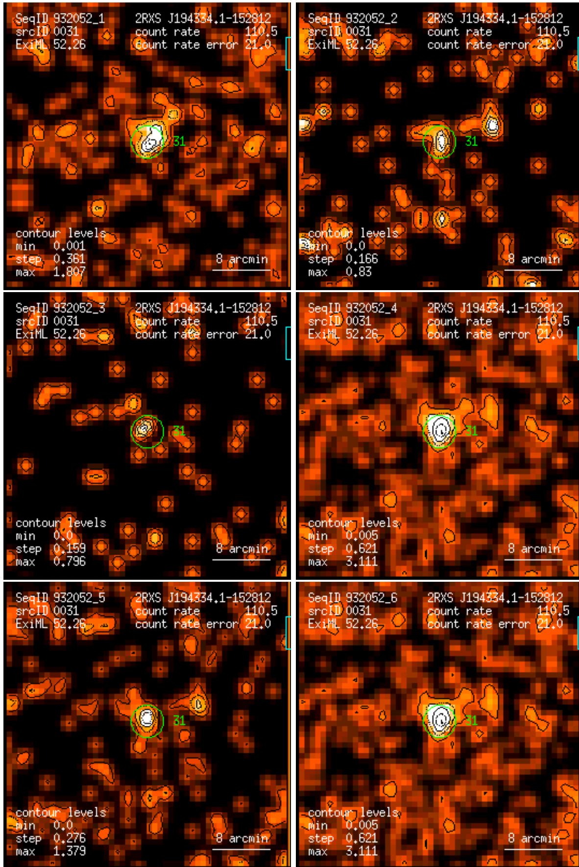
Figure 31: RASS 932052: detection 0031: band rate images, Gaussian filter: (1) PSPC channels 11 – 41, (2) 52 – 90, (3) 91 – 201, (4) 11 – 235, (5) 52 – 201, (6) 11 – 201. Broad band rates in counts/ks. Band rate contour levels in counts/ks/arcmin 2 .
