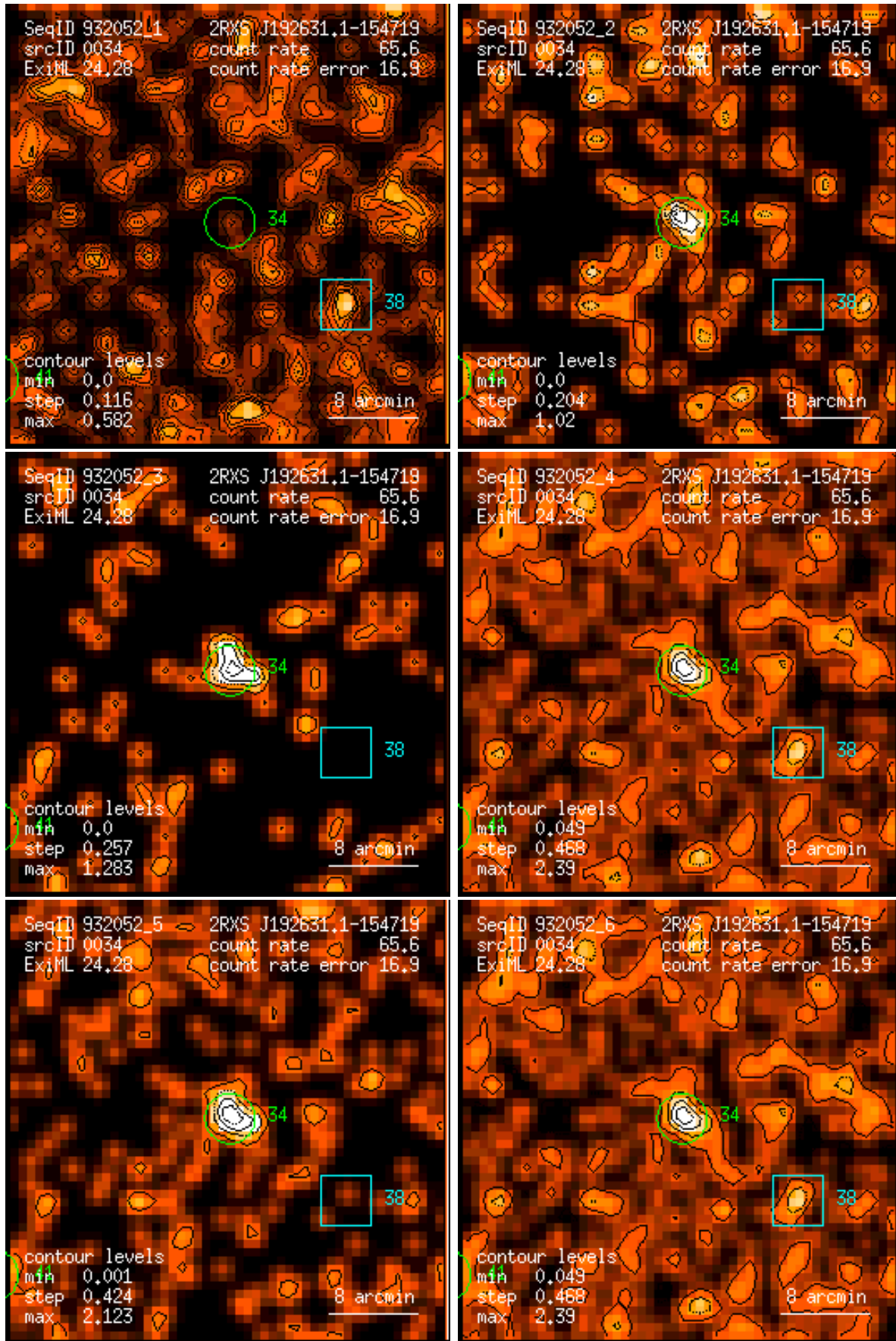
Figure 34: RASS 932052: detection 0034: band rate images, Gaussian filter: (1) PSPC channels 11 – 41, (2) 52 – 90, (3) 91 – 201, (4) 11 – 235, (5) 52 – 201, (6) 11 – 201. Broad band rates in counts/ks. Band rate contour levels in counts/ks/arcmin 2 .
