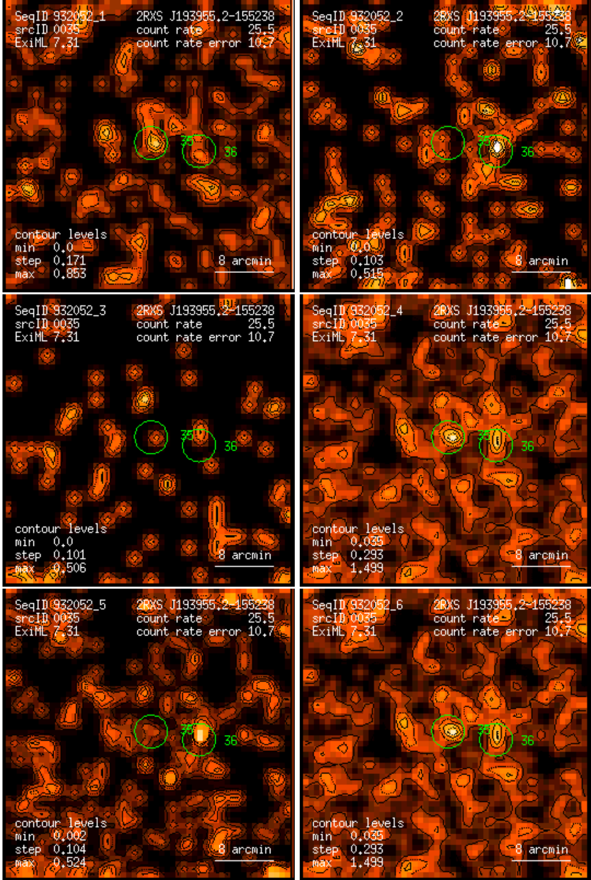
Figure 35: RASS 932052: detection 0035: band rate images, Gaussian filter: (1) PSPC channels 11 – 41, (2) 52 – 90, (3) 91 – 201, (4) 11 – 235, (5) 52 – 201, (6) 11 – 201. Broad band rates in counts/ks. Band rate contour levels in counts/ks/arcmin 2 .
