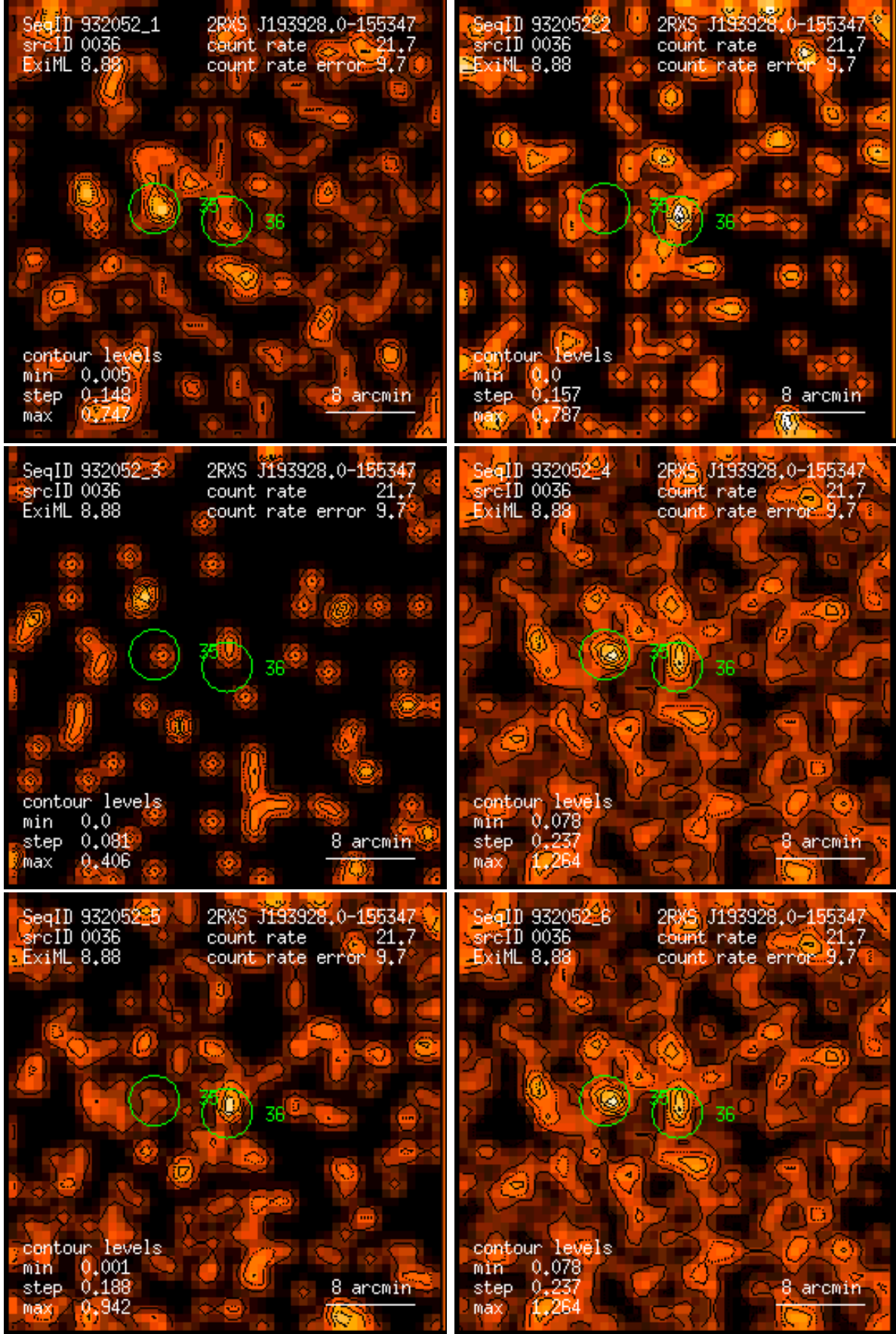
Figure 36: RASS 932052: detection 0036: band rate images, Gaussian filter: (1) PSPC channels 11 – 41, (2) 52 – 90, (3) 91 – 201, (4) 11 – 235, (5) 52 – 201, (6) 11 – 201. Broad band rates in counts/ks. Band rate contour levels in counts/ks/arcmin 2 .
