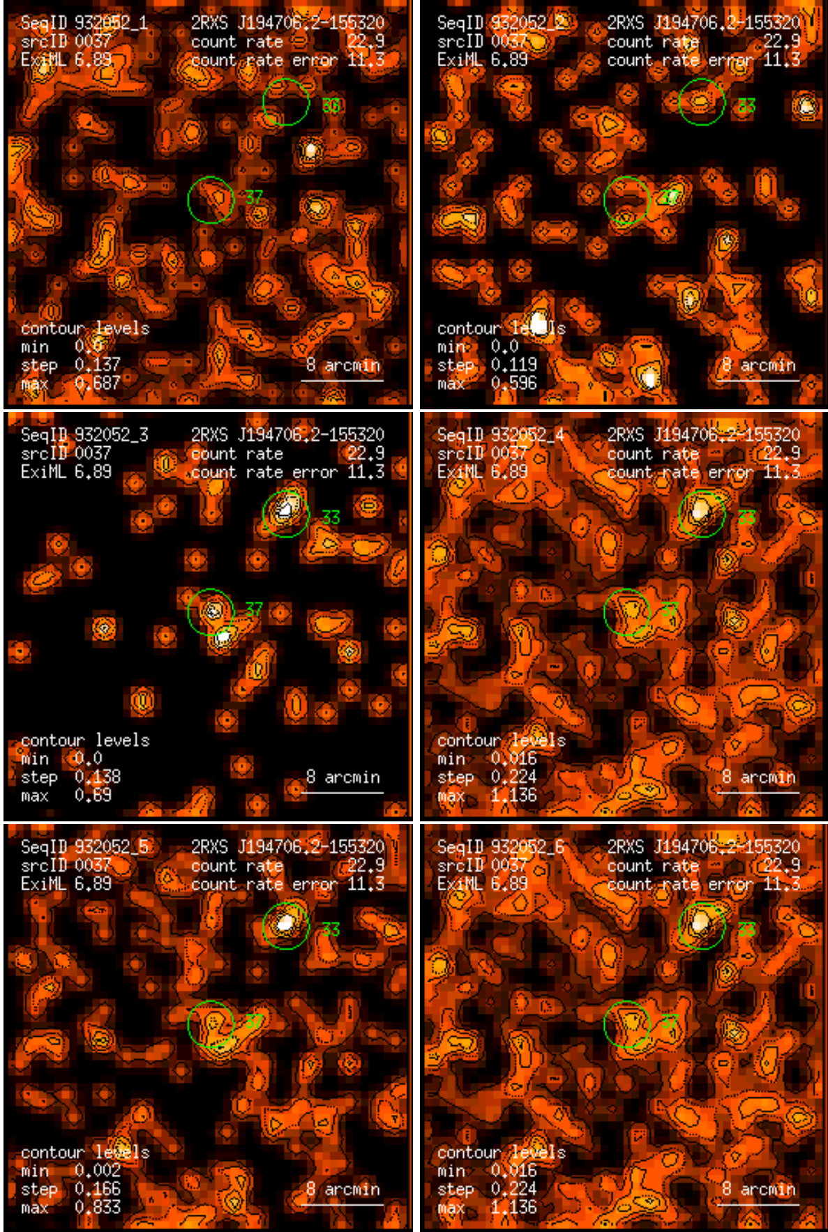
Figure 37: RASS 932052: detection 0037: band rate images, Gaussian filter: (1) PSPC channels 11 – 41, (2) 52 – 90, (3) 91 – 201, (4) 11 – 235, (5) 52 – 201, (6) 11 – 201. Broad band rates in counts/ks. Band rate contour levels in counts/ks/arcmin 2 .
