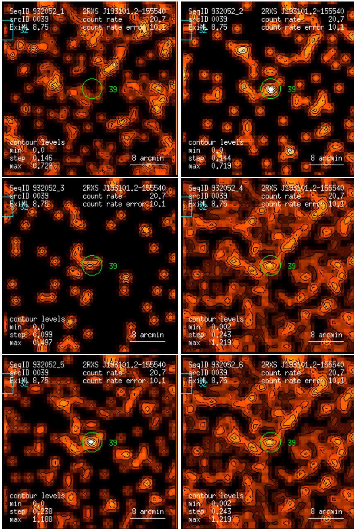
Figure 39: RASS 932052: detection 0039: band rate images, Gaussian filter: (1) PSPC channels 11 – 41, (2) 52 – 90, (3) 91 – 201, (4) 11 – 235, (5) 52 – 201, (6) 11 – 201. Broad band rates in counts/ks. Band rate contour levels in counts/ks/arcmin 2 .
