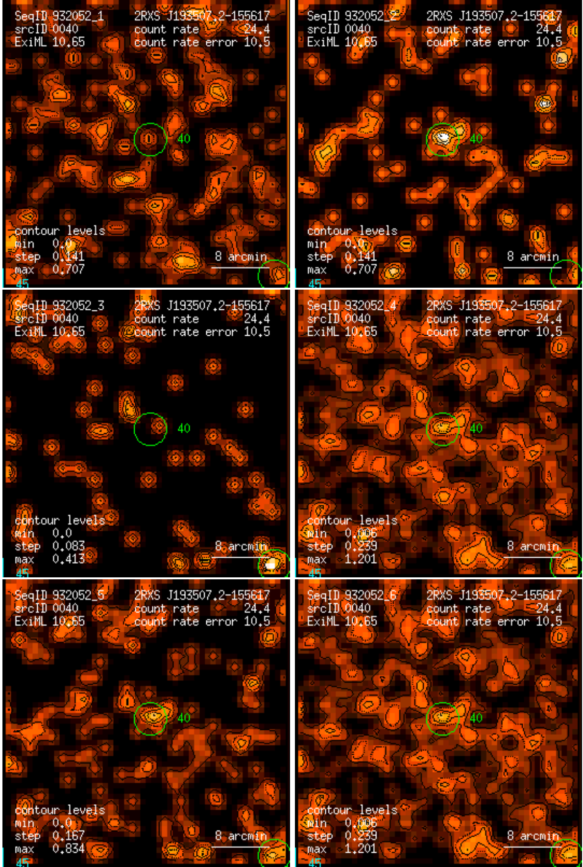
Figure 40: RASS 932052: detection 0040: band rate images, Gaussian filter: (1) PSPC channels 11 – 41, (2) 52 – 90, (3) 91 – 201, (4) 11 – 235, (5) 52 – 201, (6) 11 – 201. Broad band rates in counts/ks. Band rate contour levels in counts/ks/arcmin 2 .
