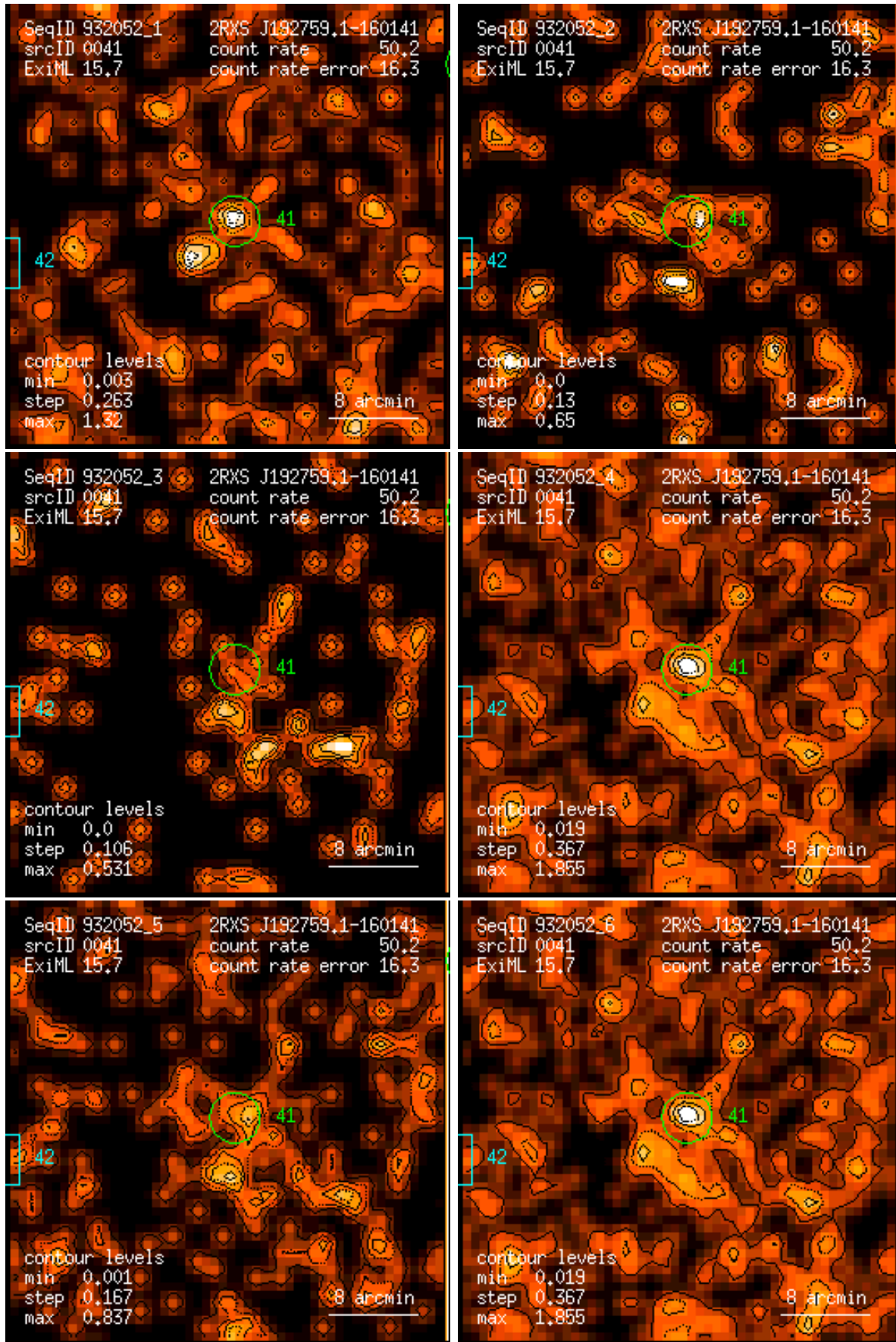
Figure 41: RASS 932052: detection 0041: band rate images, Gaussian filter: (1) PSPC channels 11 – 41, (2) 52 – 90, (3) 91 – 201, (4) 11 – 235, (5) 52 – 201, (6) 11 – 201. Broad band rates in counts/ks. Band rate contour levels in counts/ks/arcmin 2 .
