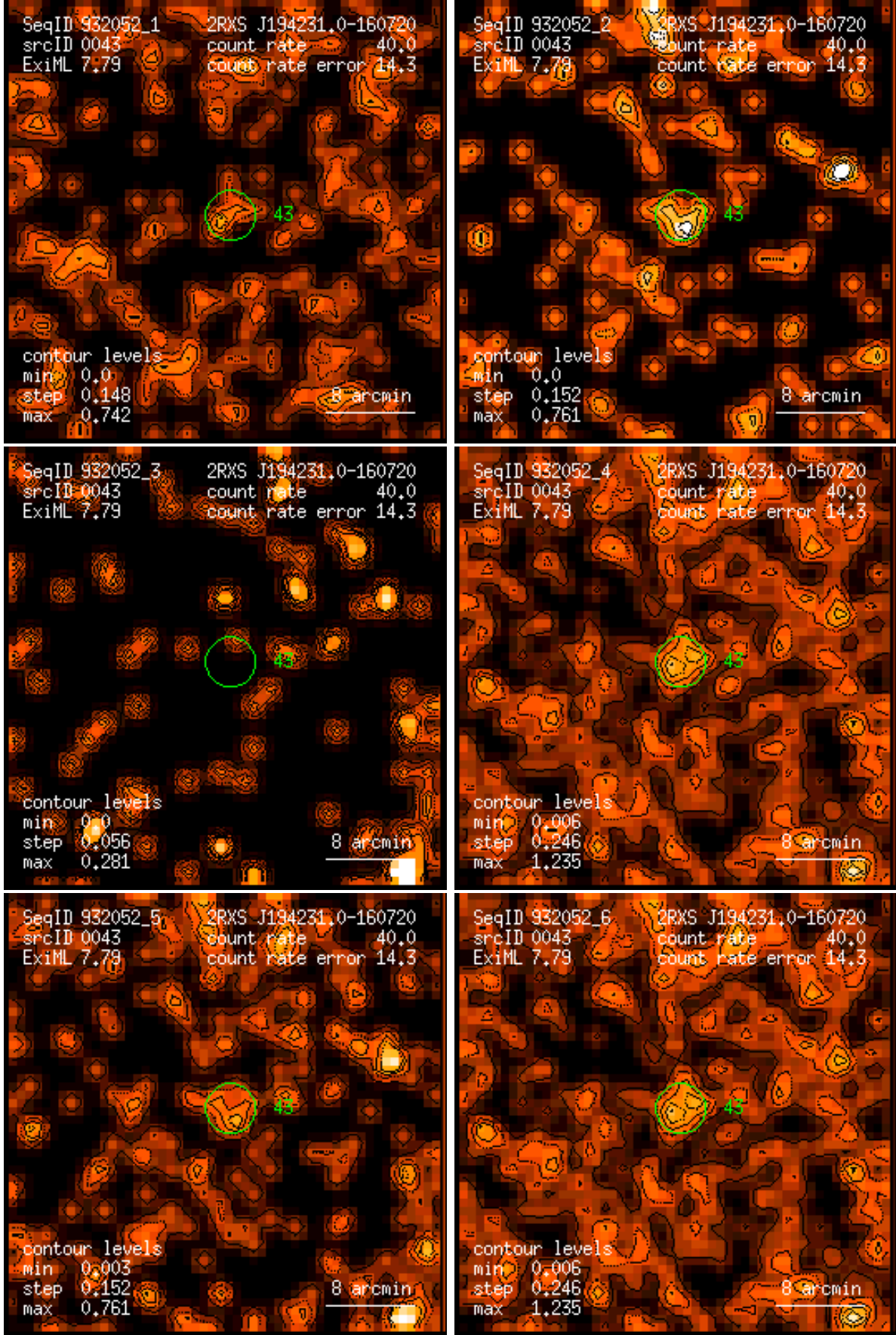
Figure 43: RASS 932052: detection 0043: band rate images, Gaussian filter: (1) PSPC channels 11 – 41, (2) 52 – 90, (3) 91 – 201, (4) 11 – 235, (5) 52 – 201, (6) 11 – 201. Broad band rates in counts/ks. Band rate contour levels in counts/ks/arcmin 2 .
