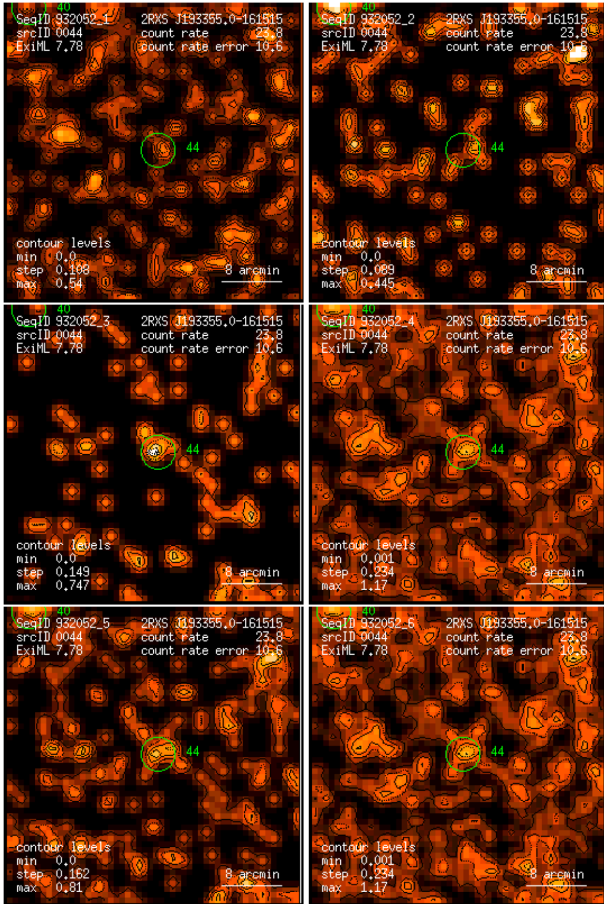
Figure 44: RASS 932052: detection 0044: band rate images, Gaussian filter: (1) PSPC channels 11 – 41, (2) 52 – 90, (3) 91 – 201, (4) 11 – 235, (5) 52 – 201, (6) 11 – 201. Broad band rates in counts/ks. Band rate contour levels in counts/ks/arcmin 2 .
