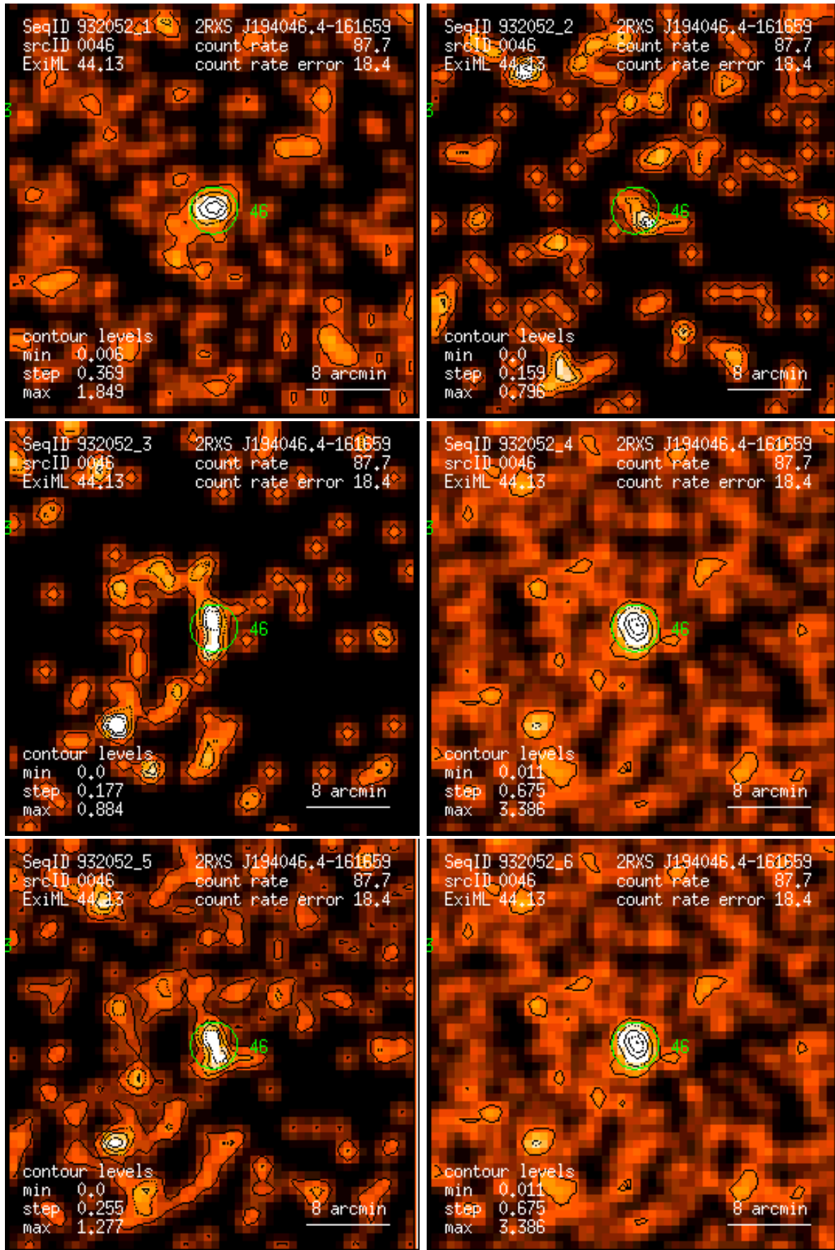
Figure 46: RASS 932052: detection 0046: band rate images, Gaussian filter: (1) PSPC channels 11 – 41, (2) 52 – 90, (3) 91 – 201, (4) 11 – 235, (5) 52 – 201, (6) 11 – 201. Broad band rates in counts/ks. Band rate contour levels in counts/ks/arcmin 2 .
