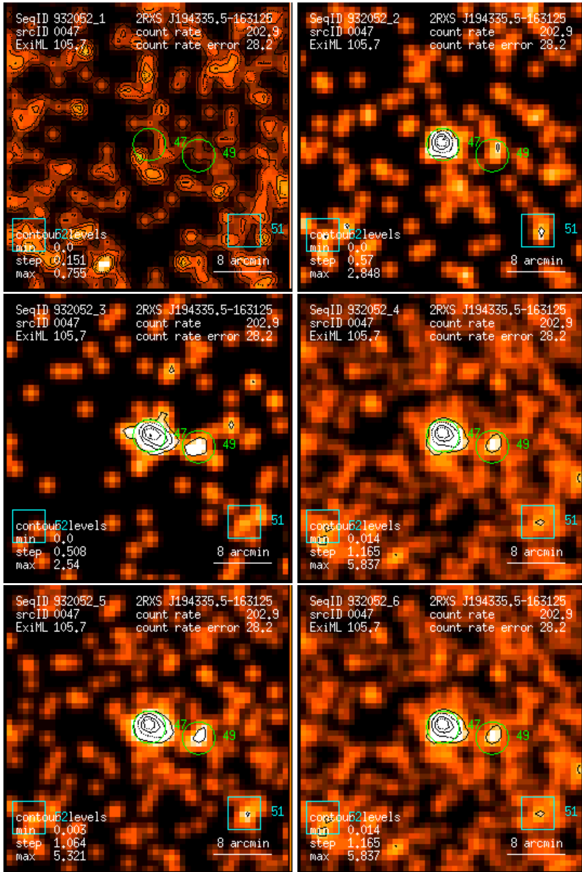
Figure 47: RASS 932052: detection 0047: band rate images, Gaussian filter: (1) PSPC channels 11 – 41, (2) 52 – 90, (3) 91 – 201, (4) 11 – 235, (5) 52 – 201, (6) 11 – 201. Broad band rates in counts/ks. Band rate contour levels in counts/ks/arcmin 2 .
