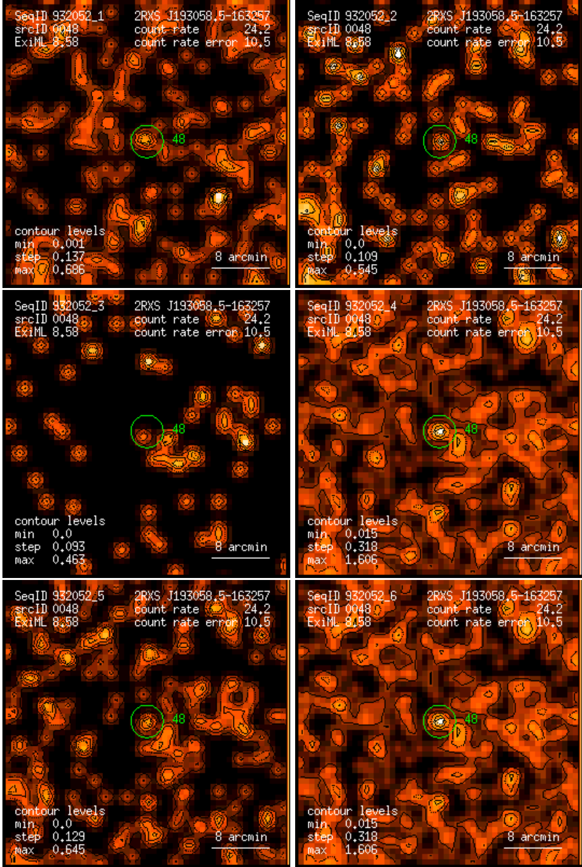
Figure 48: RASS 932052: detection 0048: band rate images, Gaussian filter: (1) PSPC channels 11 – 41, (2) 52 – 90, (3) 91 – 201, (4) 11 – 235, (5) 52 – 201, (6) 11 – 201. Broad band rates in counts/ks. Band rate contour levels in counts/ks/arcmin 2 .
