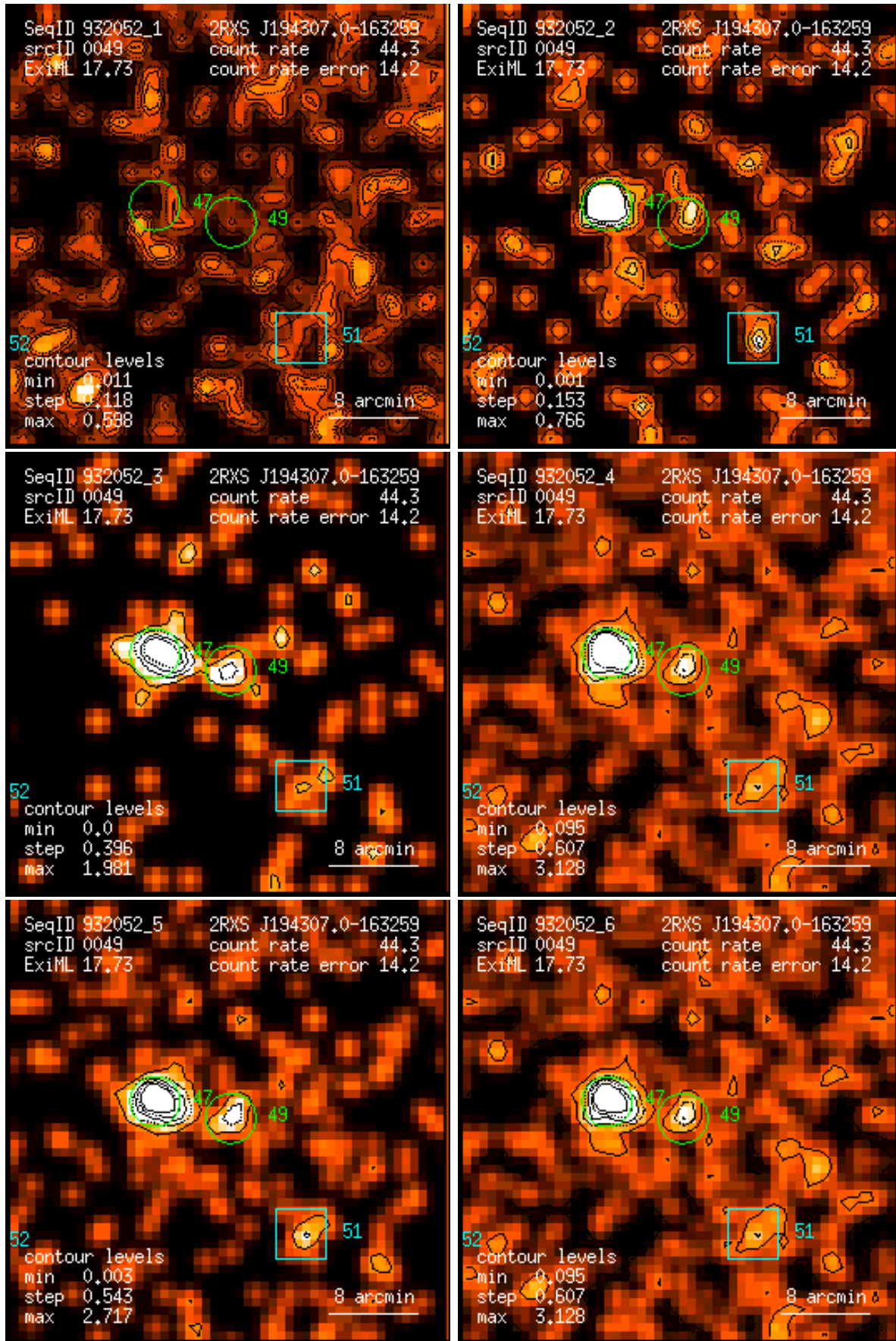
Figure 49: RASS 932052: detection 0049: band rate images, Gaussian filter: (1) PSPC channels 11 – 41, (2) 52 – 90, (3) 91 – 201, (4) 11 – 235, (5) 52 – 201, (6) 11 – 201. Broad band rates in counts/ks. Band rate contour levels in counts/ks/arcmin 2 .
