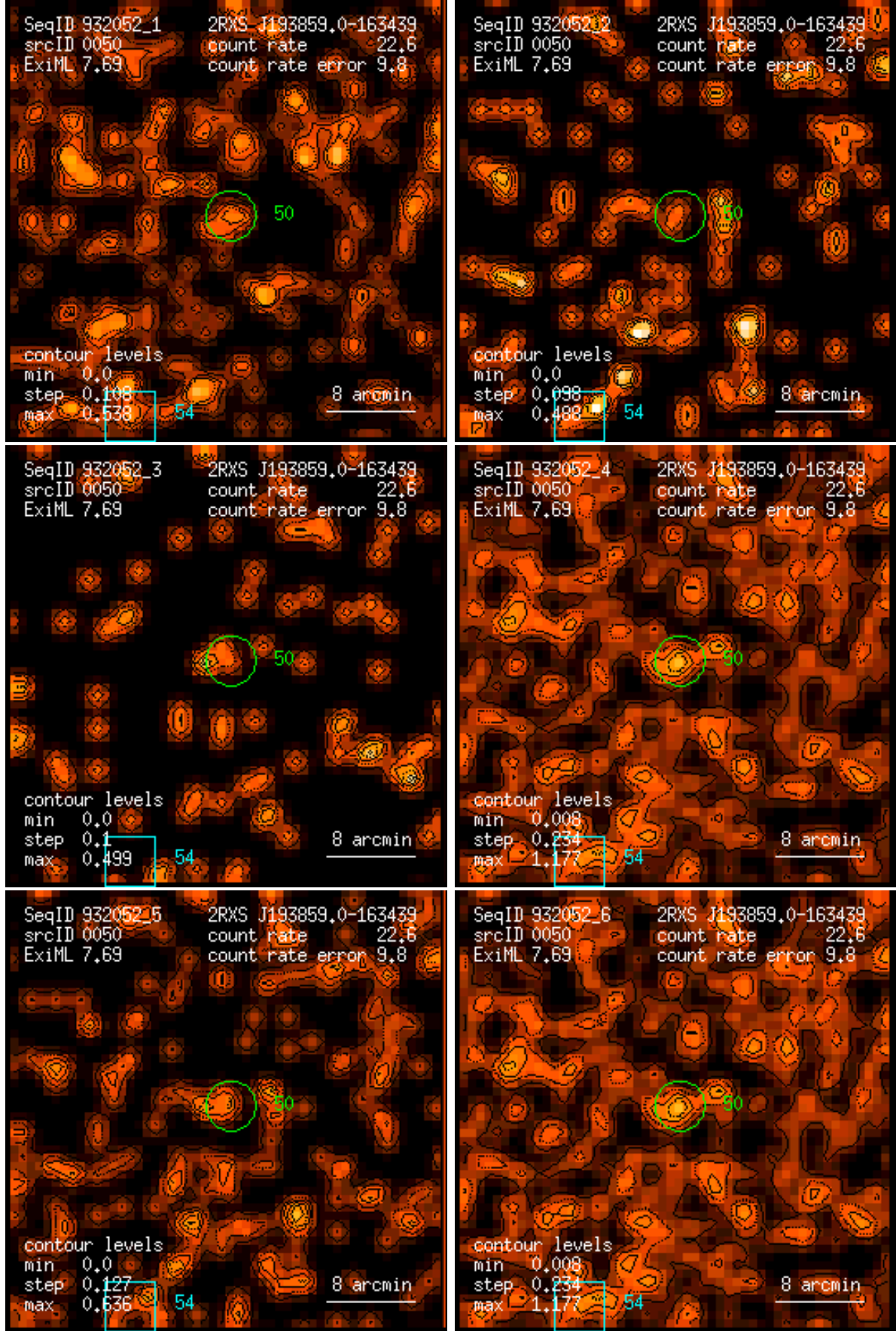
Figure 50: RASS 932052: detection 0050: band rate images, Gaussian filter: (1) PSPC channels 11 – 41, (2) 52 – 90, (3) 91 – 201, (4) 11 – 235, (5) 52 – 201, (6) 11 – 201. Broad band rates in counts/ks. Band rate contour levels in counts/ks/arcmin 2 .
