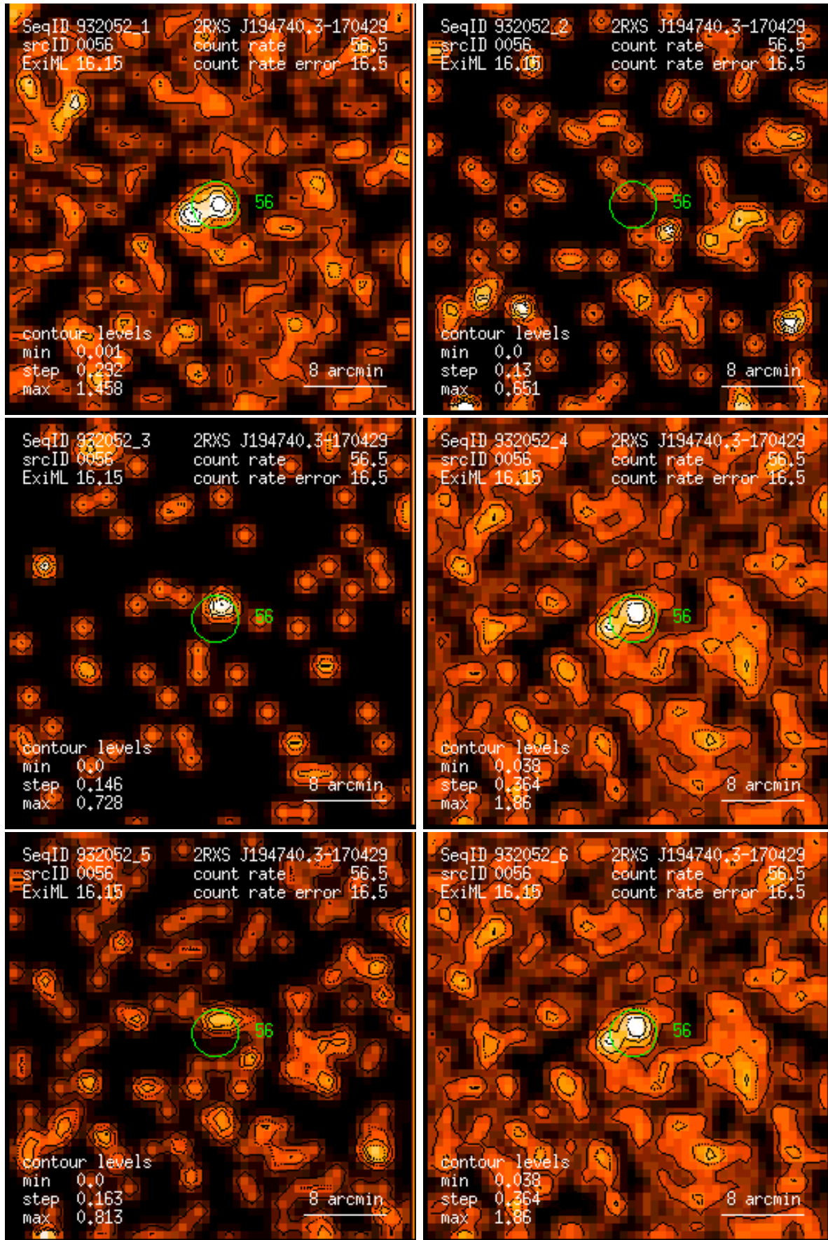
Figure 56: RASS 932052: detection 0056: band rate images, Gaussian filter: (1) PSPC channels 11 – 41, (2) 52 – 90, (3) 91 – 201, (4) 11 – 235, (5) 52 – 201, (6) 11 – 201. Broad band rates in counts/ks. Band rate contour levels in counts/ks/arcmin 2 .
