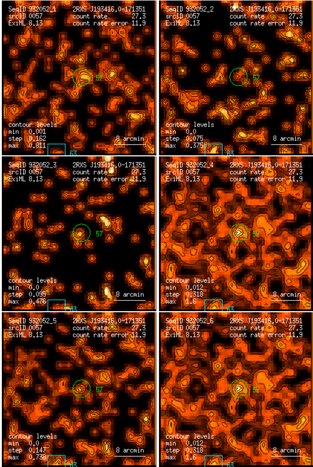
Figure 57: RASS 932052: detection 0057: band rate images, Gaussian filter: (1) PSPC channels 11 – 41, (2) 52 – 90, (3) 91 – 201, (4) 11 – 235, (5) 52 – 201, (6) 11 – 201. Broad band rates in counts/ks. Band rate contour levels in counts/ks/arcmin 2 .
