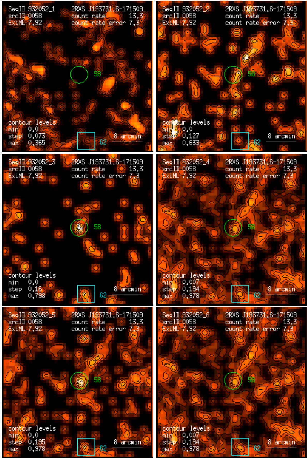
Figure 58: RASS 932052: detection 0058: band rate images, Gaussian filter: (1) PSPC channels 11 – 41, (2) 52 – 90, (3) 91 – 201, (4) 11 – 235, (5) 52 – 201, (6) 11 – 201. Broad band rates in counts/ks. Band rate contour levels in counts/ks/arcmin 2 .
