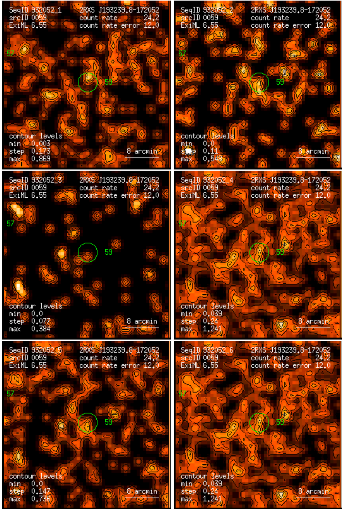
Figure 59: RASS 932052: detection 0059: band rate images, Gaussian filter: (1) PSPC channels 11 – 41, (2) 52 – 90, (3) 91 – 201, (4) 11 – 235, (5) 52 – 201, (6) 11 – 201. Broad band rates in counts/ks. Band rate contour levels in counts/ks/arcmin 2 .
