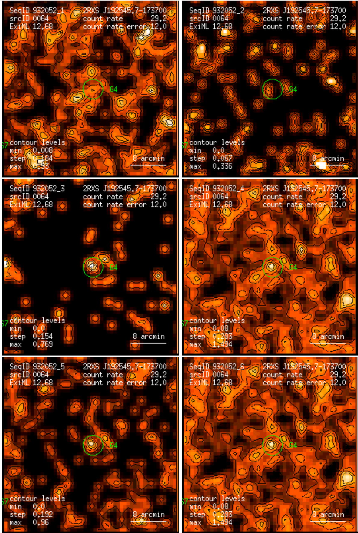
Figure 64: RASS 932052: detection 0064: band rate images, Gaussian filter: (1) PSPC channels 11 – 41, (2) 52 – 90, (3) 91 – 201, (4) 11 – 235, (5) 52 – 201, (6) 11 – 201. Broad band rates in counts/ks. Band rate contour levels in counts/ks/arcmin 2 .
