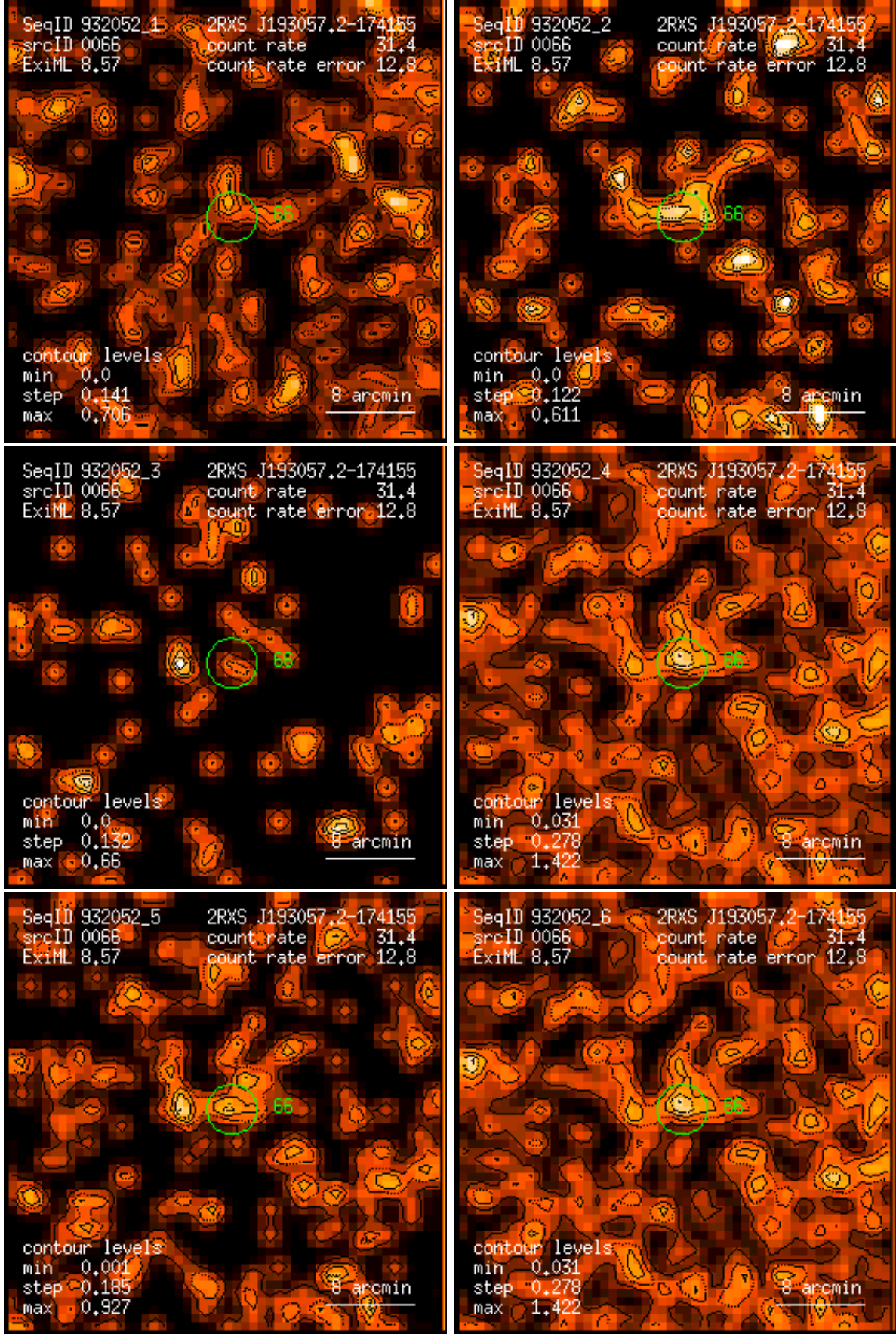
Figure 66: RASS 932052: detection 0066: band rate images, Gaussian filter: (1) PSPC channels 11 – 41, (2) 52 – 90, (3) 91 – 201, (4) 11 – 235, (5) 52 – 201, (6) 11 – 201. Broad band rates in counts/ks. Band rate contour levels in counts/ks/arcmin 2 .
