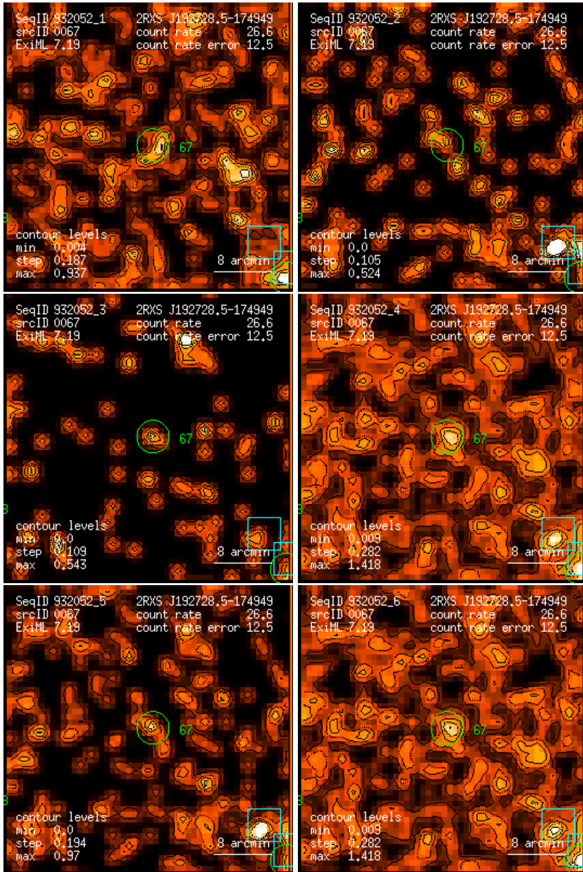
Figure 67: RASS 932052: detection 0067: band rate images, Gaussian filter: (1) PSPC channels 11 – 41, (2) 52 – 90, (3) 91 – 201, (4) 11 – 235, (5) 52 – 201, (6) 11 – 201. Broad band rates in counts/ks. Band rate contour levels in counts/ks/arcmin 2 .
