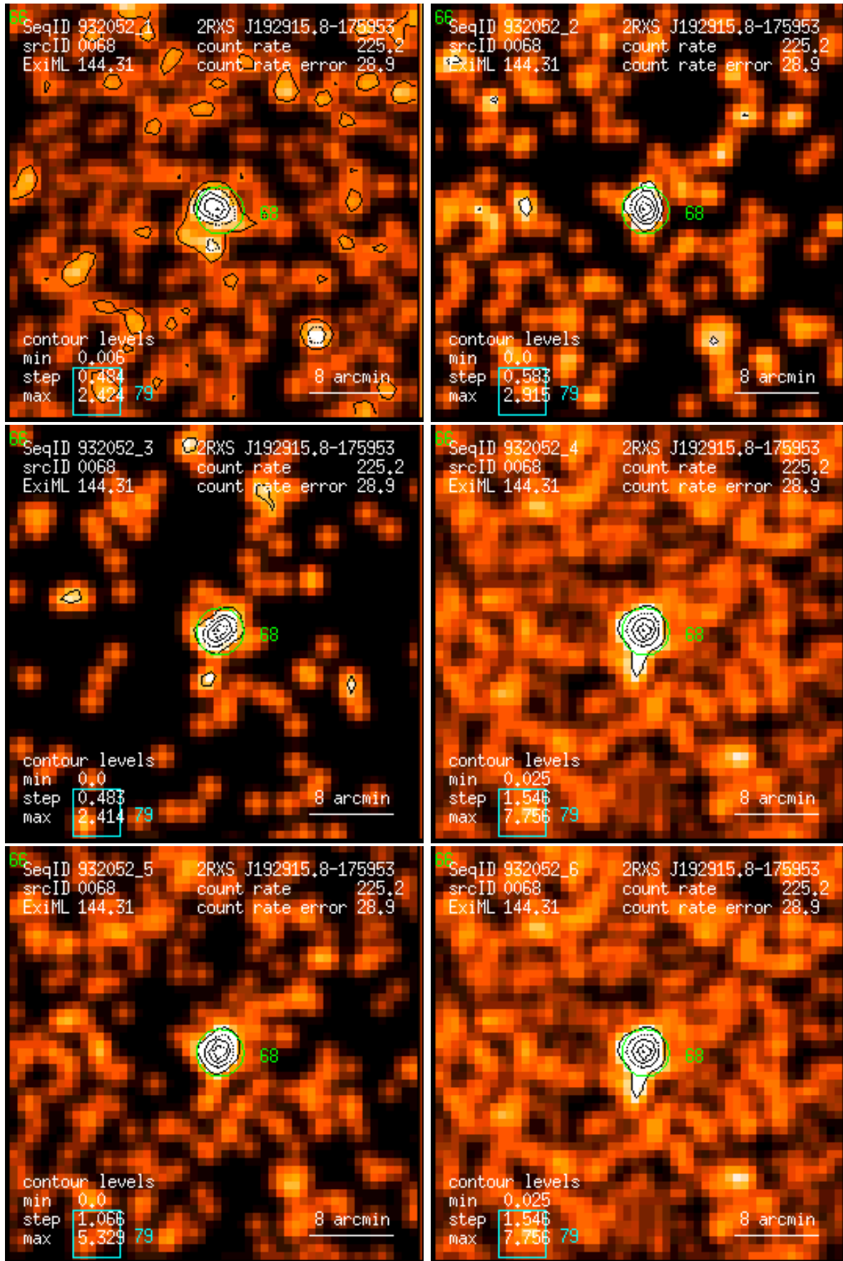
Figure 68: RASS 932052: detection 0068: band rate images, Gaussian filter: (1) PSPC channels 11 – 41, (2) 52 – 90, (3) 91 – 201, (4) 11 – 235, (5) 52 – 201, (6) 11 – 201. Broad band rates in counts/ks. Band rate contour levels in counts/ks/arcmin 2 .
