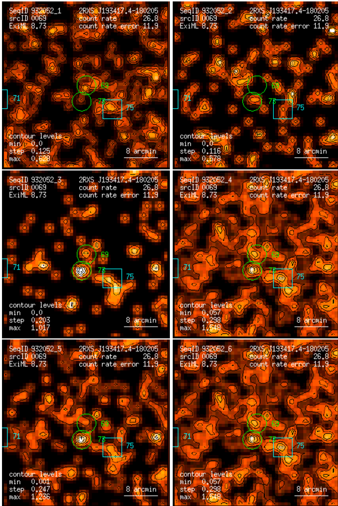
Figure 69: RASS 932052: detection 0069: band rate images, Gaussian filter: (1) PSPC channels 11 – 41, (2) 52 – 90, (3) 91 – 201, (4) 11 – 235, (5) 52 – 201, (6) 11 – 201. Broad band rates in counts/ks. Band rate contour levels in counts/ks/arcmin 2 .
