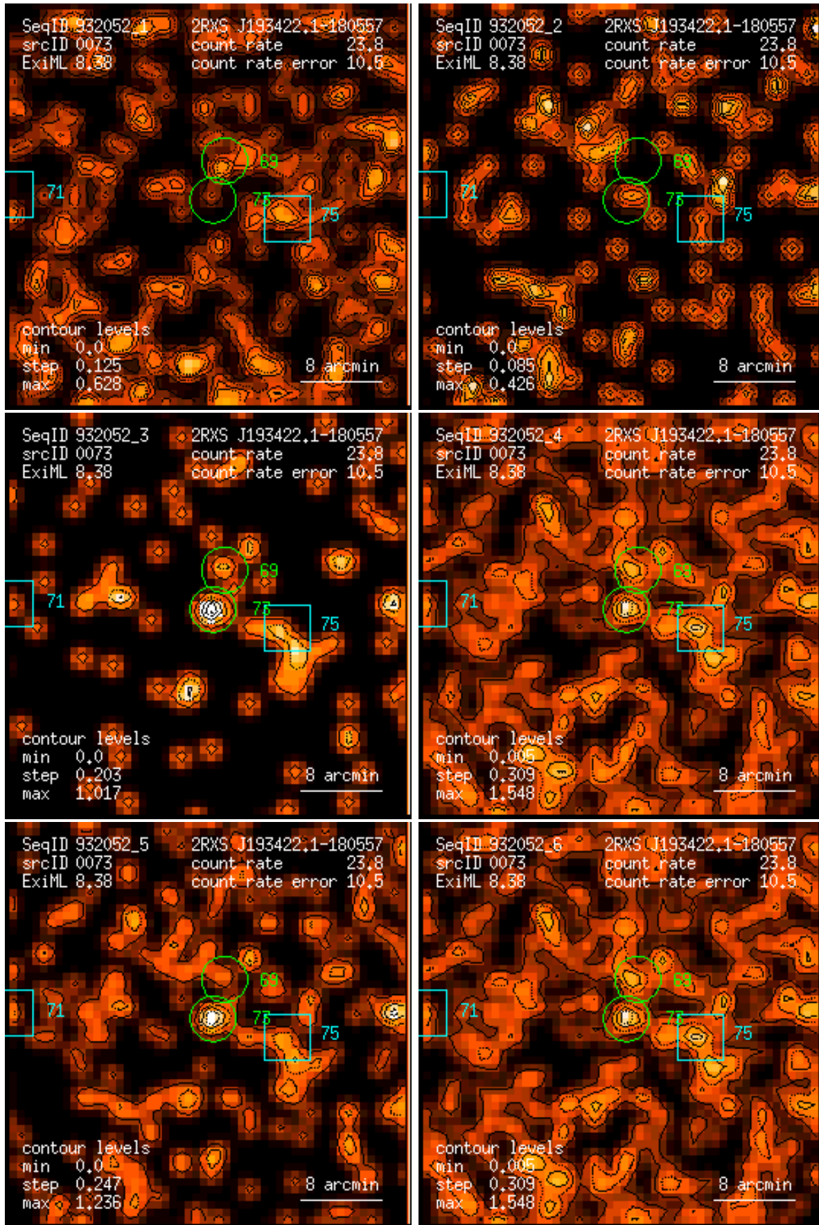
Figure 73: RASS 932052: detection 0073: band rate images, Gaussian filter: (1) PSPC channels 11 – 41, (2) 52 – 90, (3) 91 – 201, (4) 11 – 235, (5) 52 – 201, (6) 11 – 201. Broad band rates in counts/ks. Band rate contour levels in counts/ks/arcmin 2 .
