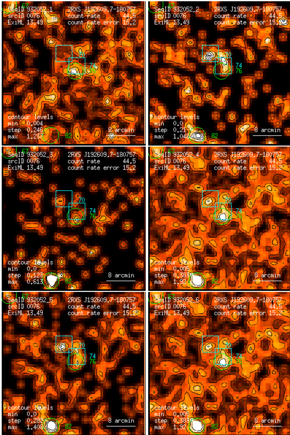
Figure 76: RASS 932052: detection 0076: band rate images, Gaussian filter: (1) PSPC channels 11 – 41, (2) 52 – 90, (3) 91 – 201, (4) 11 – 235, (5) 52 – 201, (6) 11 – 201. Broad band rates in counts/ks. Band rate contour levels in counts/ks/arcmin 2 .
