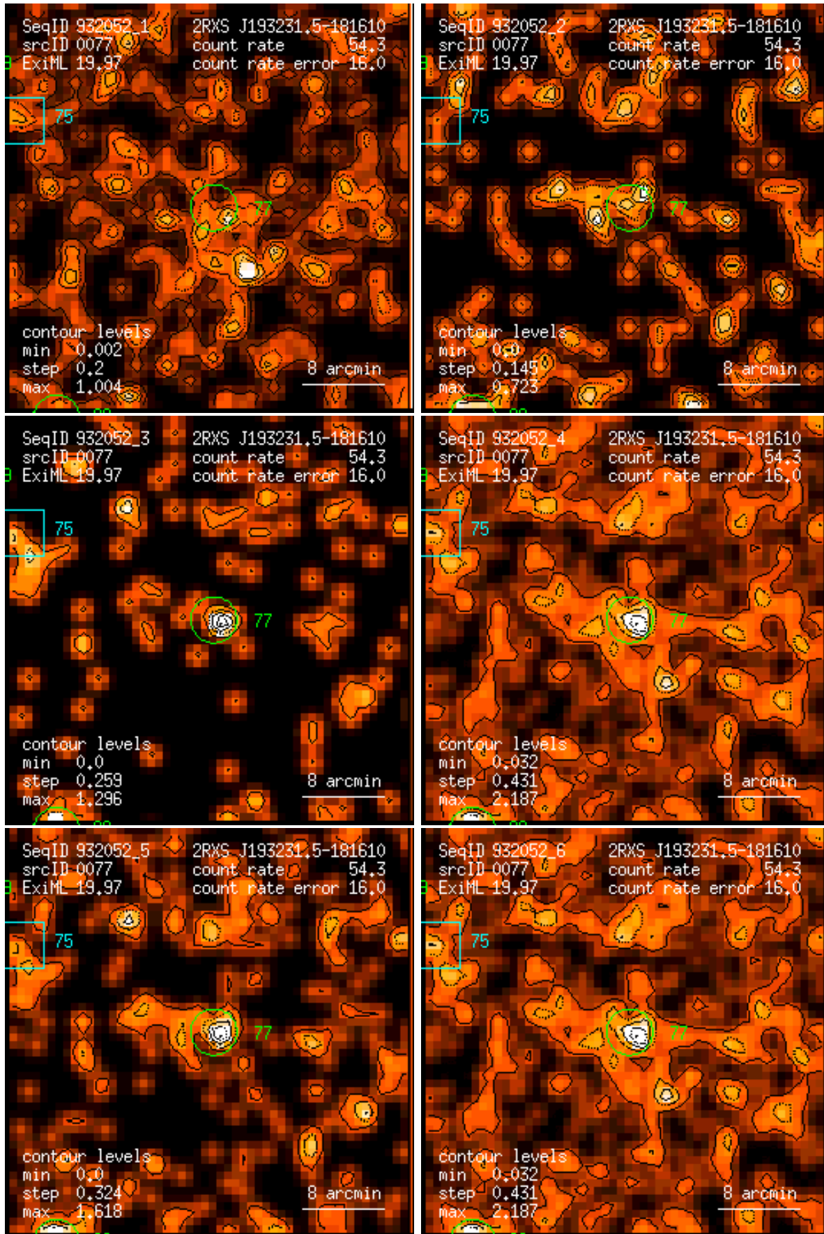
Figure 77: RASS 932052: detection 0077: band rate images, Gaussian filter: (1) PSPC channels 11 – 41, (2) 52 – 90, (3) 91 – 201, (4) 11 – 235, (5) 52 – 201, (6) 11 – 201. Broad band rates in counts/ks. Band rate contour levels in counts/ks/arcmin 2 .
