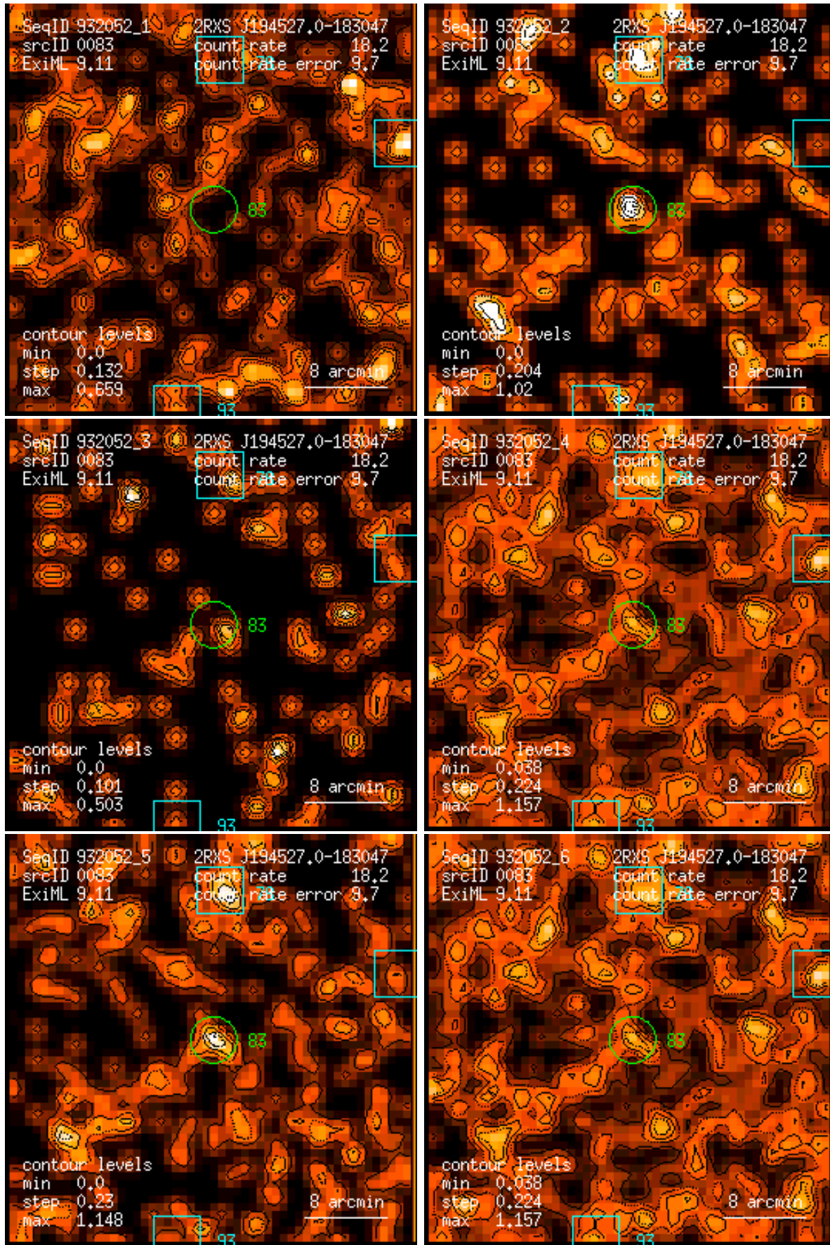
Figure 83: RASS 932052: detection 0083: band rate images, Gaussian filter: (1) PSPC channels 11 – 41, (2) 52 – 90, (3) 91 – 201, (4) 11 – 235, (5) 52 – 201, (6) 11 – 201. Broad band rates in counts/ks. Band rate contour levels in counts/ks/arcmin 2 .
