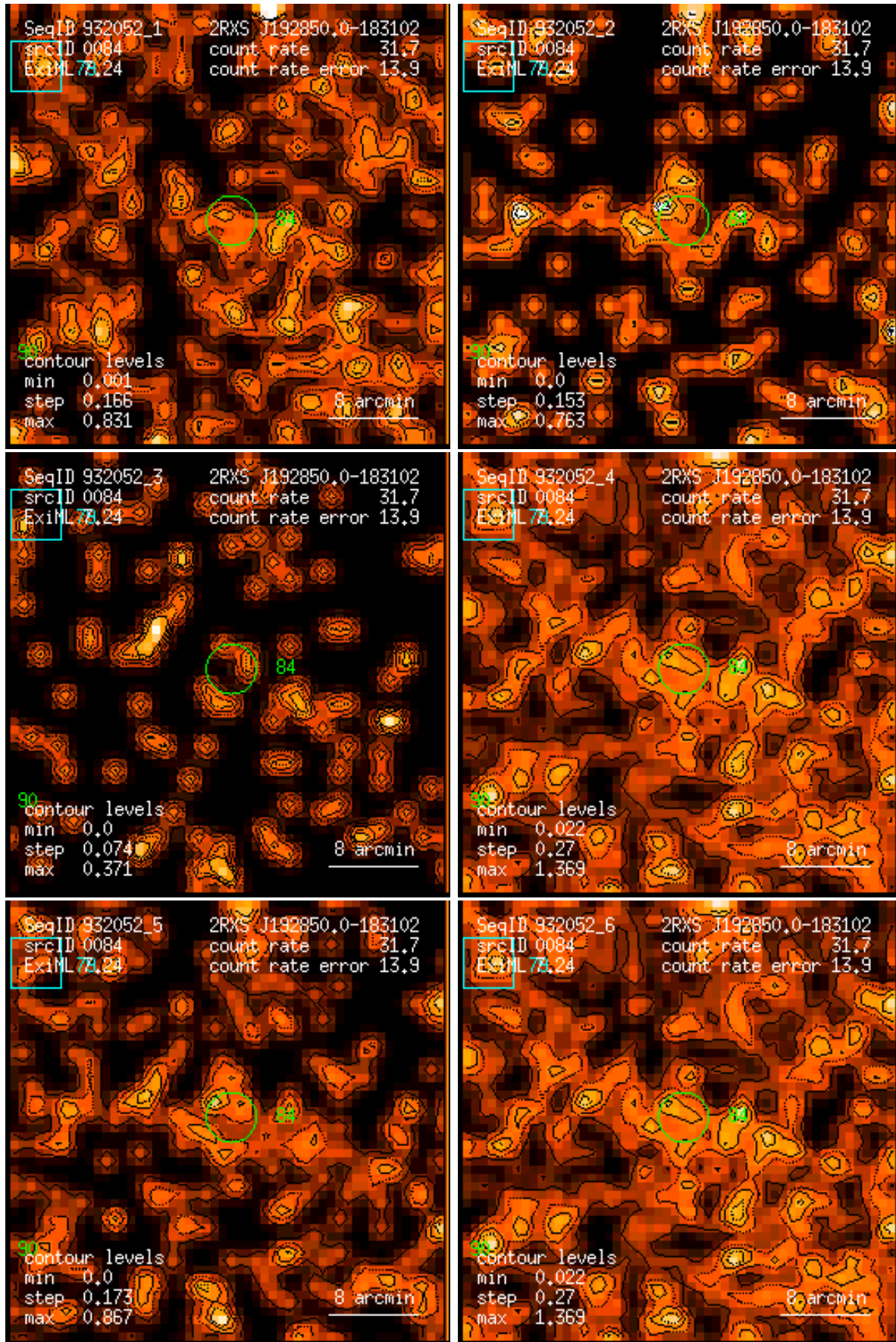
Figure 84: RASS 932052: detection 0084: band rate images, Gaussian filter: (1) PSPC channels 11 – 41, (2) 52 – 90, (3) 91 – 201, (4) 11 – 235, (5) 52 – 201, (6) 11 – 201. Broad band rates in counts/ks. Band rate contour levels in counts/ks/arcmin 2 .
