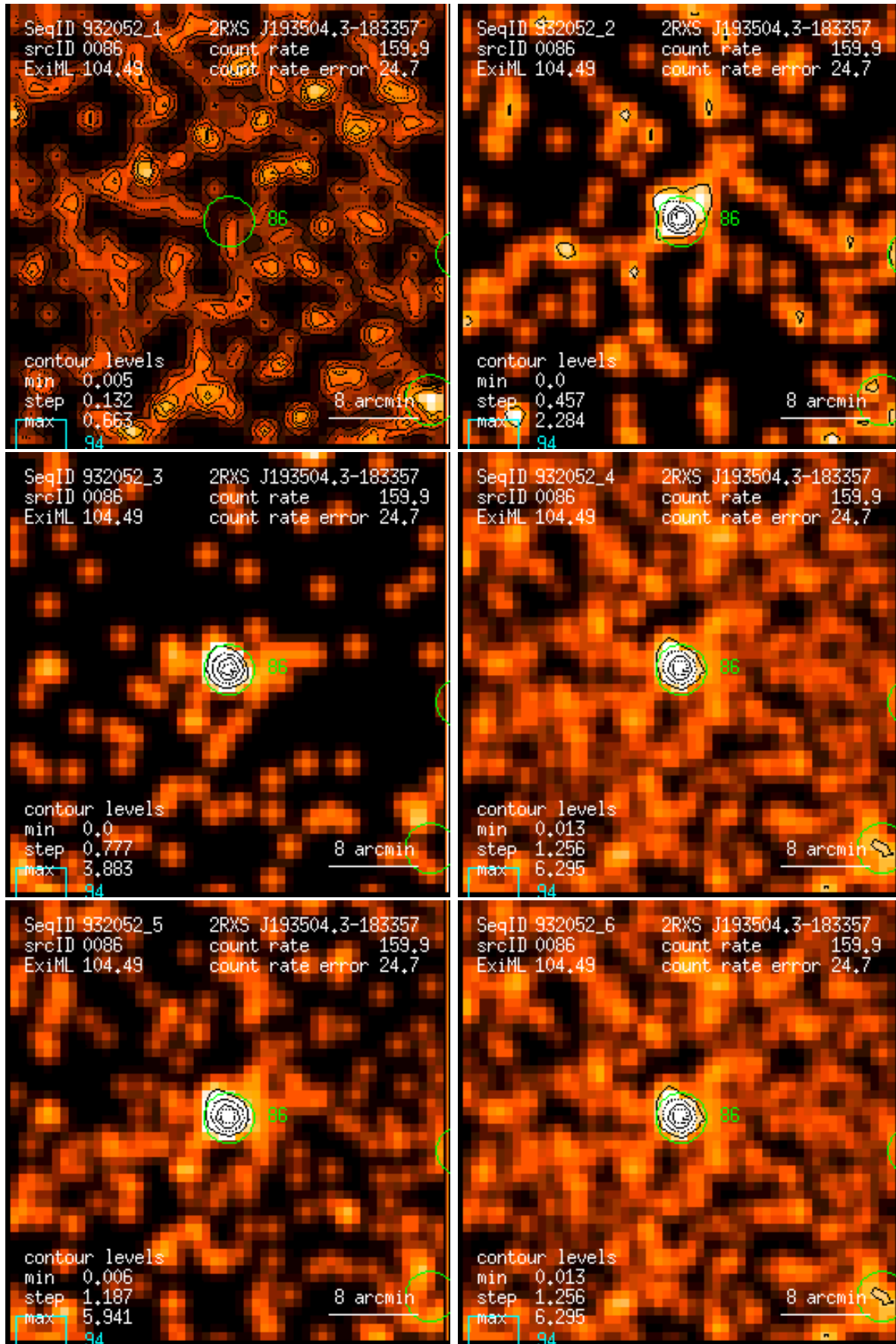
Figure 86: RASS 932052: detection 0086: band rate images, Gaussian filter: (1) PSPC channels 11 – 41, (2) 52 – 90, (3) 91 – 201, (4) 11 – 235, (5) 52 – 201, (6) 11 – 201. Broad band rates in counts/ks. Band rate contour levels in counts/ks/arcmin 2 .
